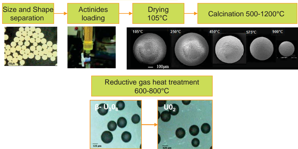
Figure 20 : Principle of the WAR process applied to Uranium dioxide based materials synthesis
