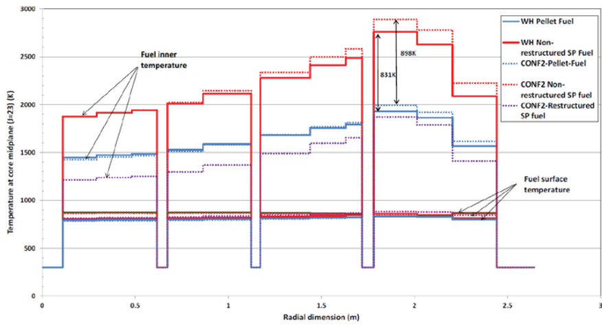
Figure 23: Map of fuel centerline and surface temperatures for different fuel loadings in the core at the very Beginning Of Life [87]
