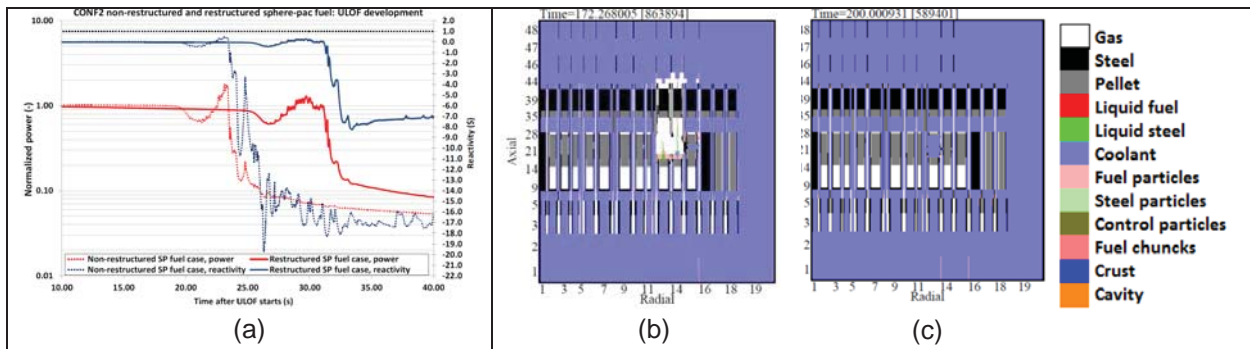
Figure 26: Behaviour of the CONF-2 core – spherepacked fuel – during ULOF conditions at BOL [87].
