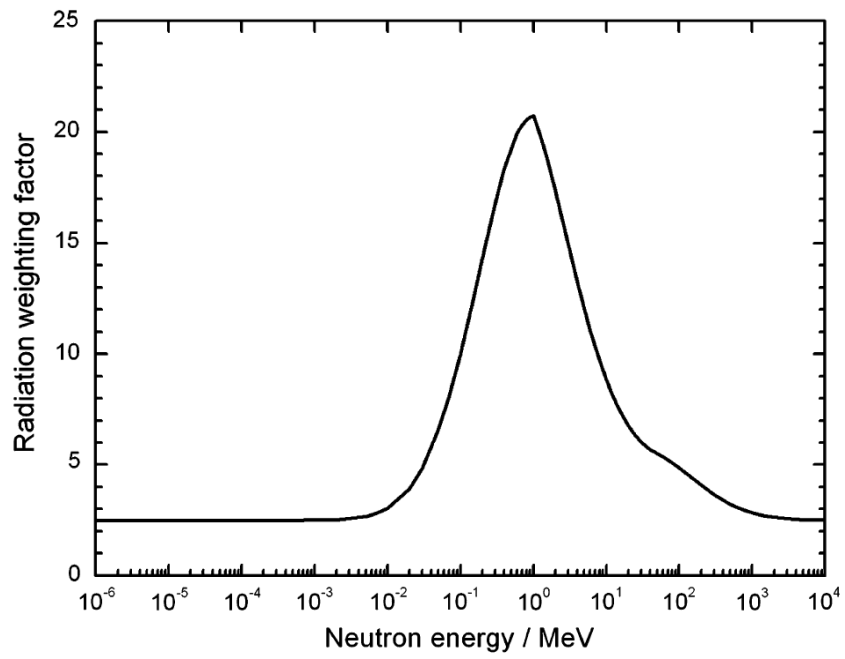
Figure: Radiation weighting factor w_R as a function of neutron energy, reproduced from ICRP 103.
