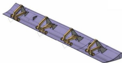
4-bar linkage kinematics
