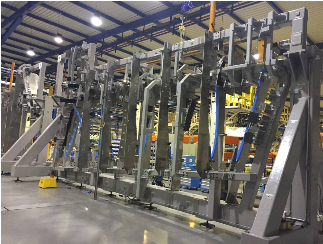
Figure 1: Main Jig
