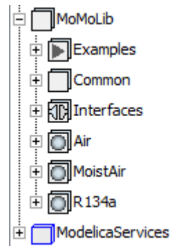
Structure of the MoMoLib media library
