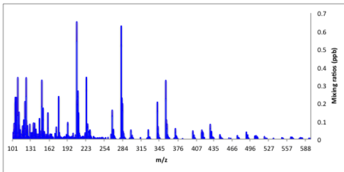
Figure 1: Mixing ratios of SVOCs ranging from m/z 100 to m/z 600 for 10L indoor sample
