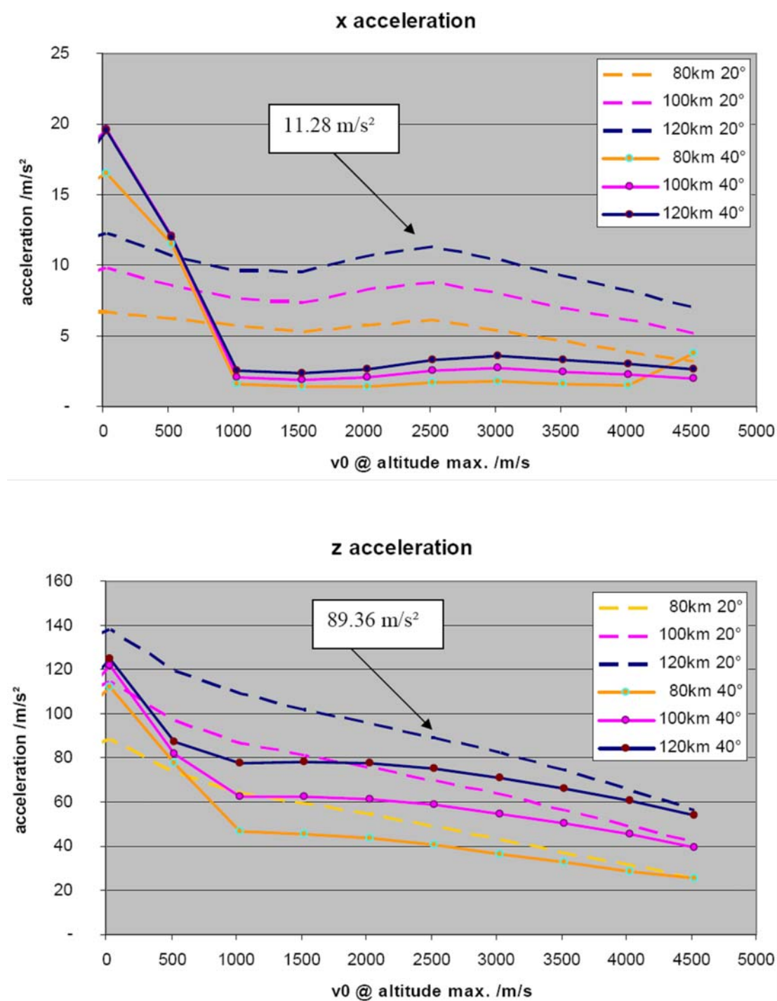
Figures: Sensitivity of the acceleration loads on horizontal speeds at maximum altitude during re-entry for a given vehicle for different maximum altitudes and angles of attack. (The numbers in the frames address reference values for accuracy control.)
