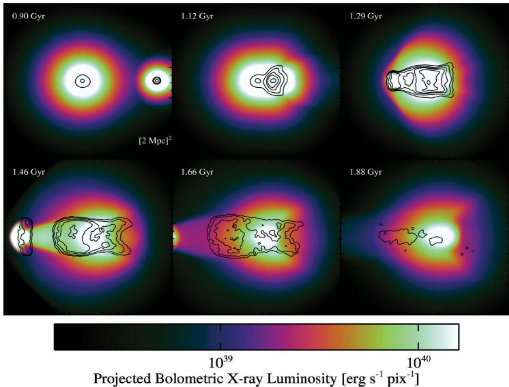
FIGURE 1 : simulated merger between galaxy clusters showing the generation of diffuse radio emission (contours). Colors are the X-ray emission (from Donnert et al. 2013).
