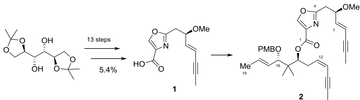
Scheme 1. Overview of the synthetic chemistry developed by the Fellow.
