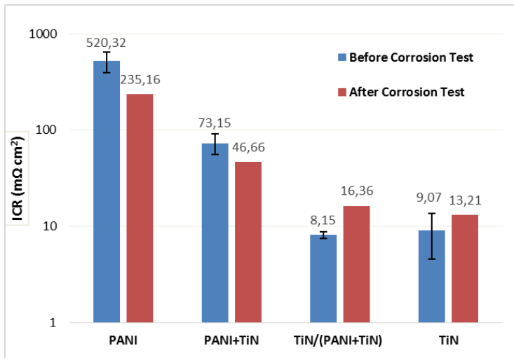
Figure 2: ICR values for various coatings before and after corrosion testing.
