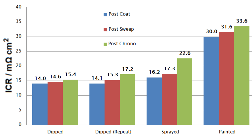
Figure 3: ICR before and after 1h at 1.4 V for coatings with variation of application method.
