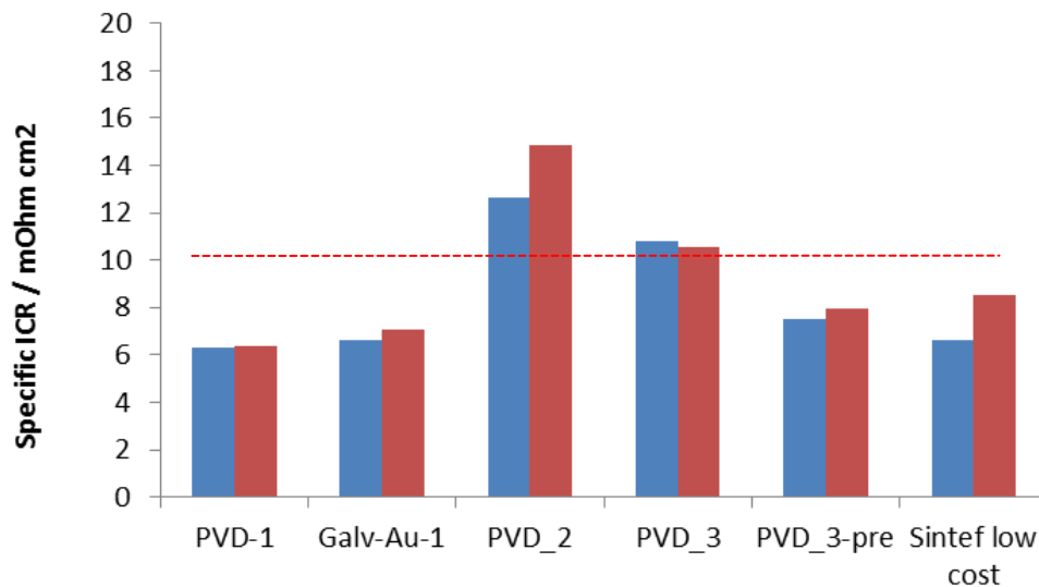
Figure 6: Specific ICR @ 166 N cm -2 (land area 6.19 cm 2 ), before and after AST.
