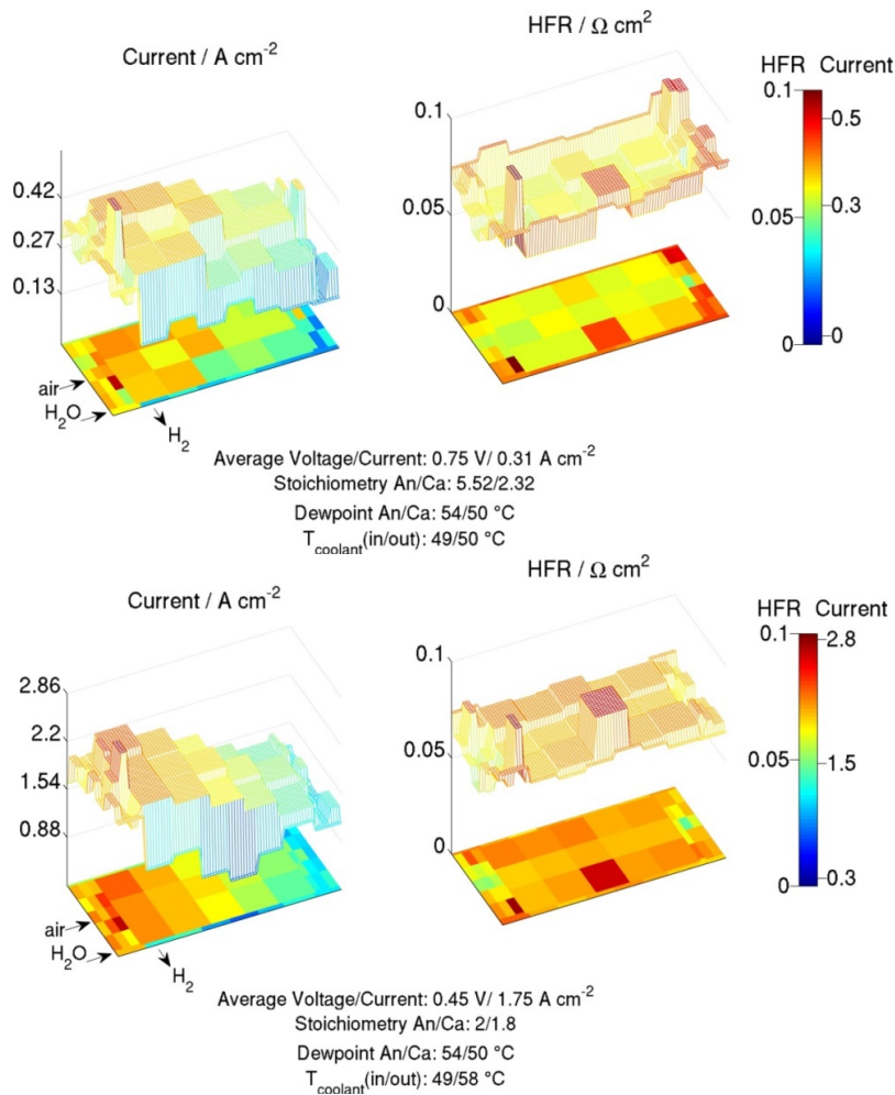
Figure 8: Current distribution at two potentiostatic points (top: 0.75V, bottom: 0.45V).
