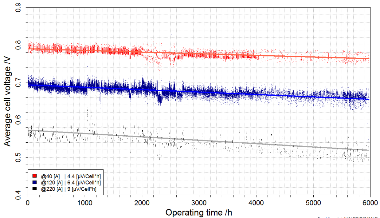
Figure 10: Voltage behaviour of the stack for three different current levels.
