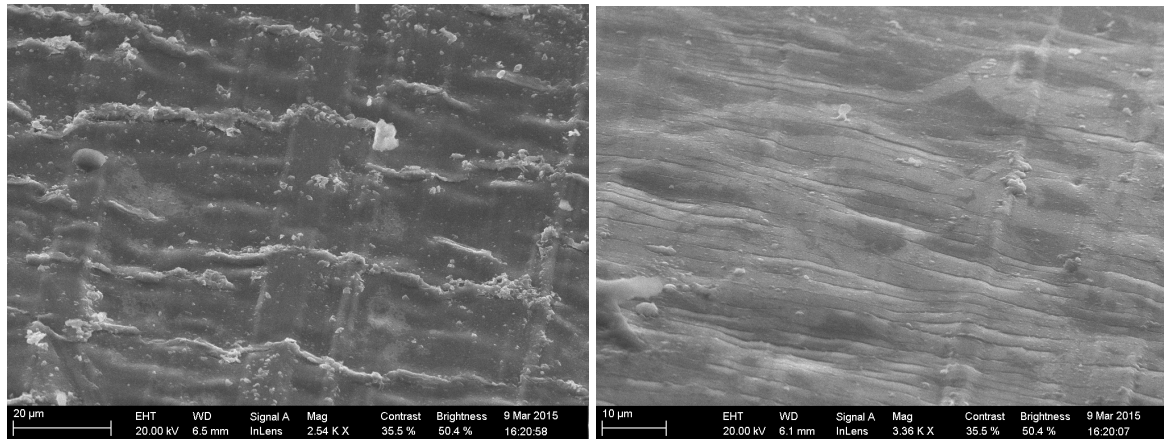
Figure 4: SEM image of a PVD pre-coated substrate after stamping, land top to the left and edge of land to the right.
