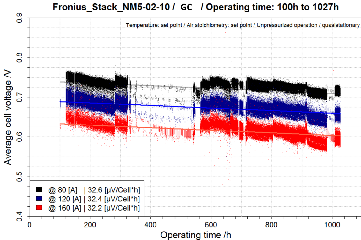
Figure 12: Degradation rate analysis over lifetime for gold coated metal BPP plate stack at different currents levels
