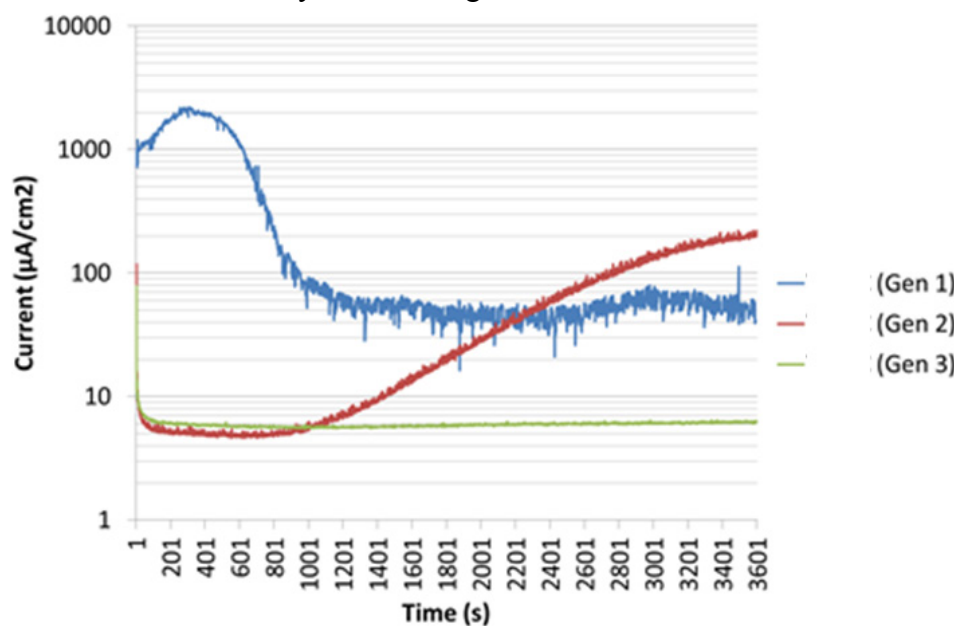
Figure 1: Potentiostatic corrosion tests at 1.4V for three generations of a PVD coating.
