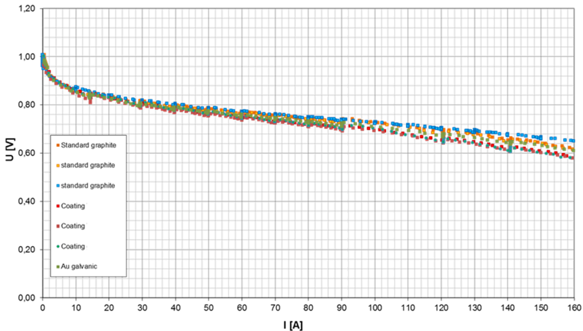
Figure 9: Current voltage curves of the cells with the different coated bipolar plates.
