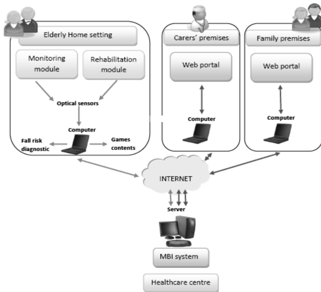
Figure 1: Architecture of the final platform and intended service.
