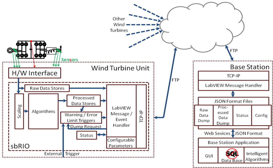
Wind TurBar System Breakdown of the Base Station and the Wind Turbine Unit Functionality
