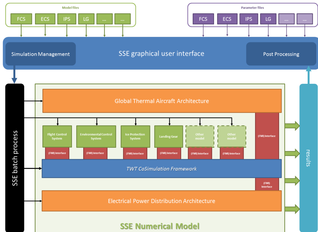
Figure 2: Architecture of the iSSE
