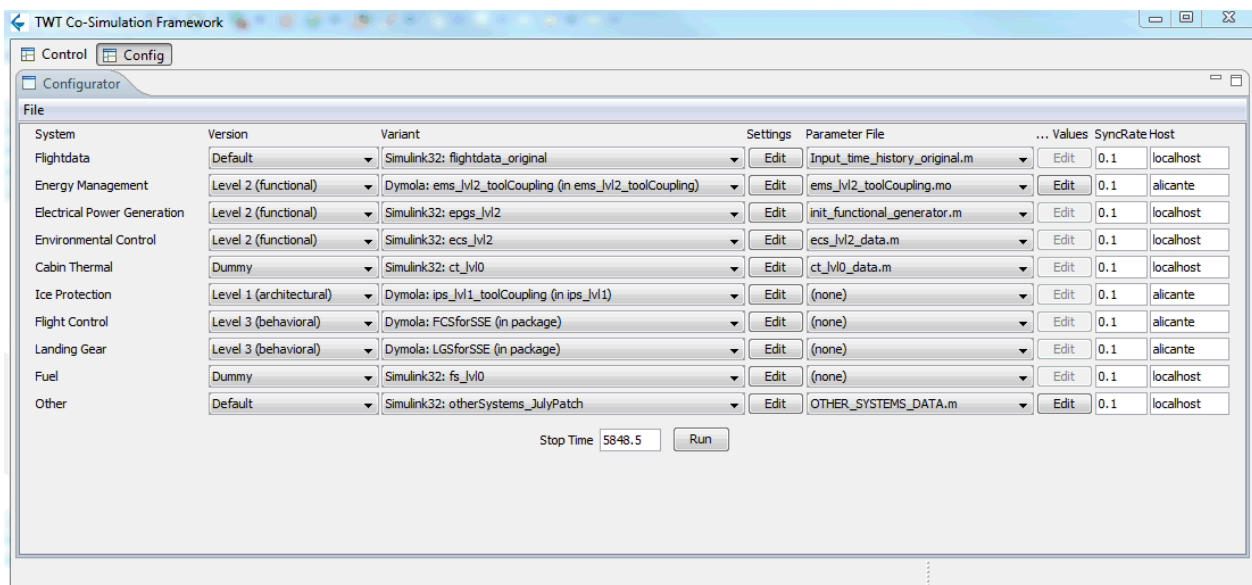
Figure 4: iSSE GUI showing an example of a co-simulation configuration
