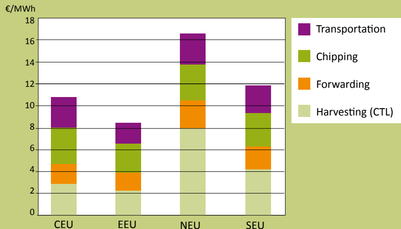
Estimated supply costs for chips from broadleaved stems from thinning. CTL=cut to length
