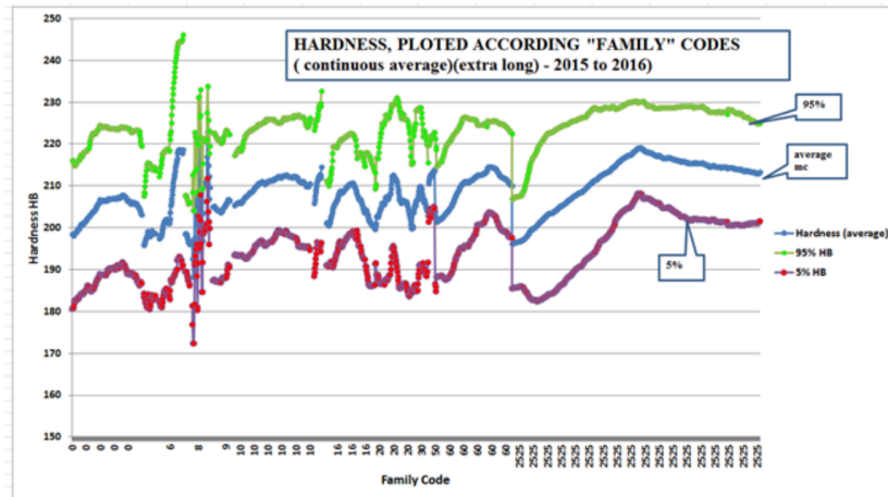
Figure nº 23.- A protocol to classify the pieces by “families”, and defining the expected characteristics (mechanical and level of defects and type), has been built up to indicate the end user and foundry the expected characteristics of a new parts, following the trend of giving global services to customer.
