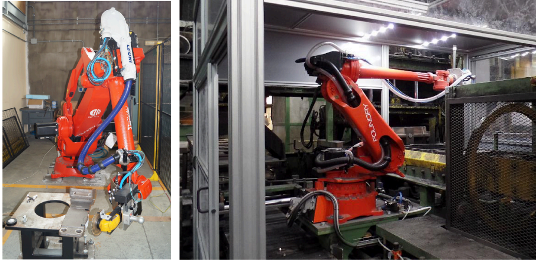
Figure n° 10.- Flexicast robotic cells (#2 and #3)
