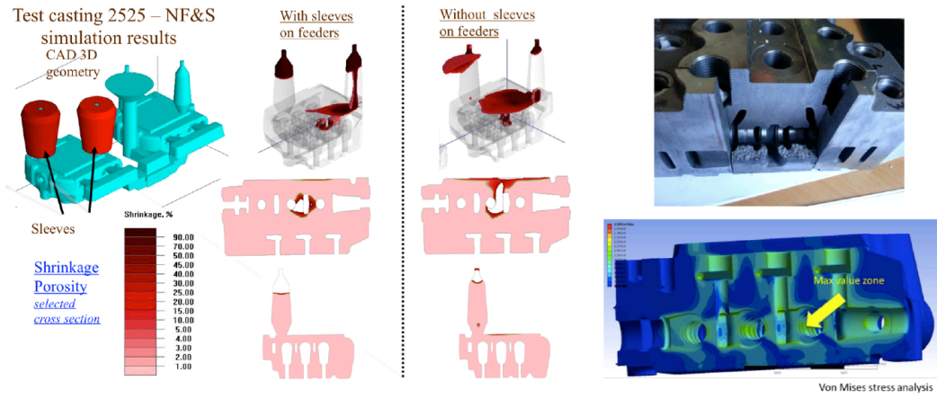
Figure n° 15.- Experimental and numerical results of specific Flexicast ref. 2525 DCV piece.
