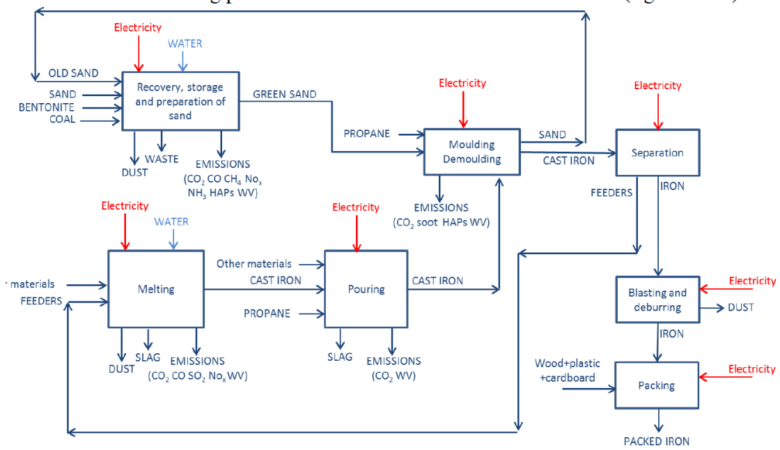
Figure n° 21.- Block diagram of the cast iron manufacturing process
