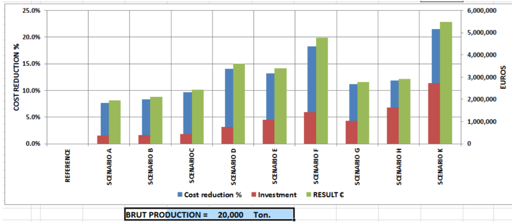
Figure n° 26.-Cost reduction, Needed Investment, and Final Result for the scenarios (20.000 Ton)
