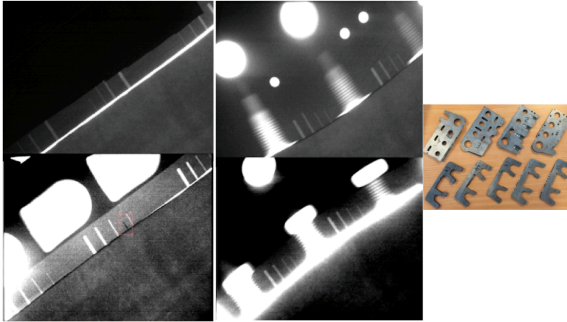
Figure nº 8.- X-ray castings inspection
