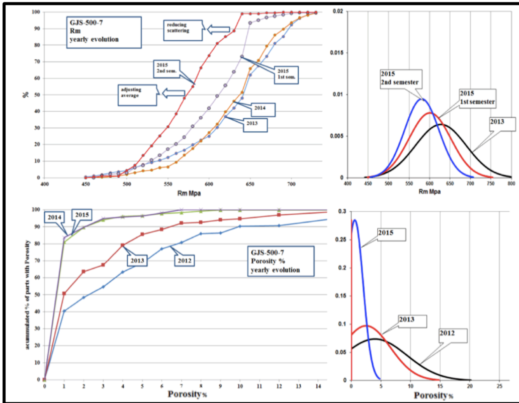
Figure nº 9.- Temporal evolution and Normal distribution of porosity (%) and Rm of GJS500-7 for annual periods (2012-2015)
