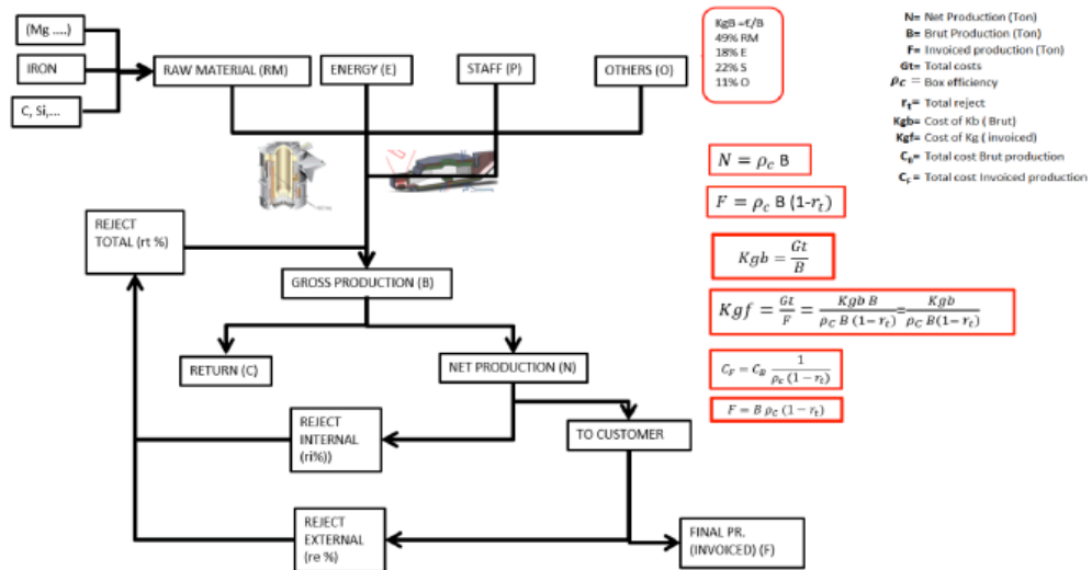
Figure n° 2.- Flow diagram of cast iron production line, from raw material to finished pieces
