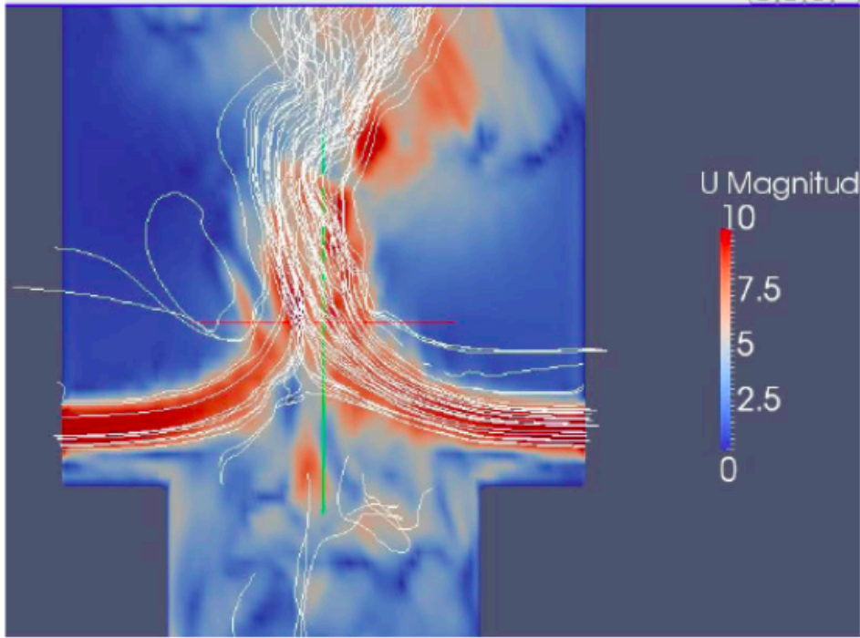
Figure nº 11: Gas flow for laminar barrier
