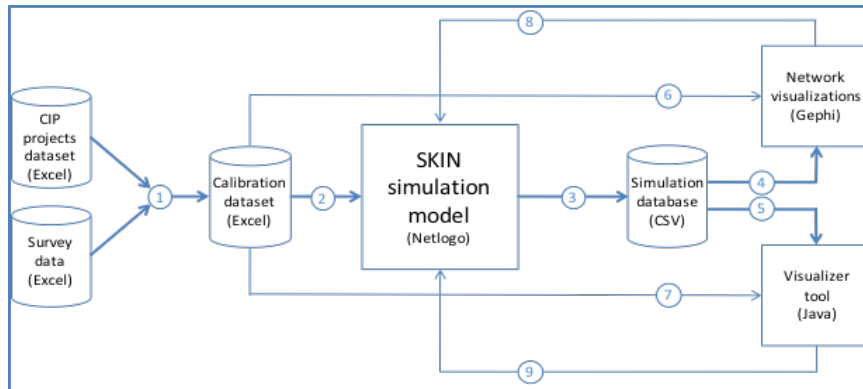
Figure 1: Great Skin Workflow
