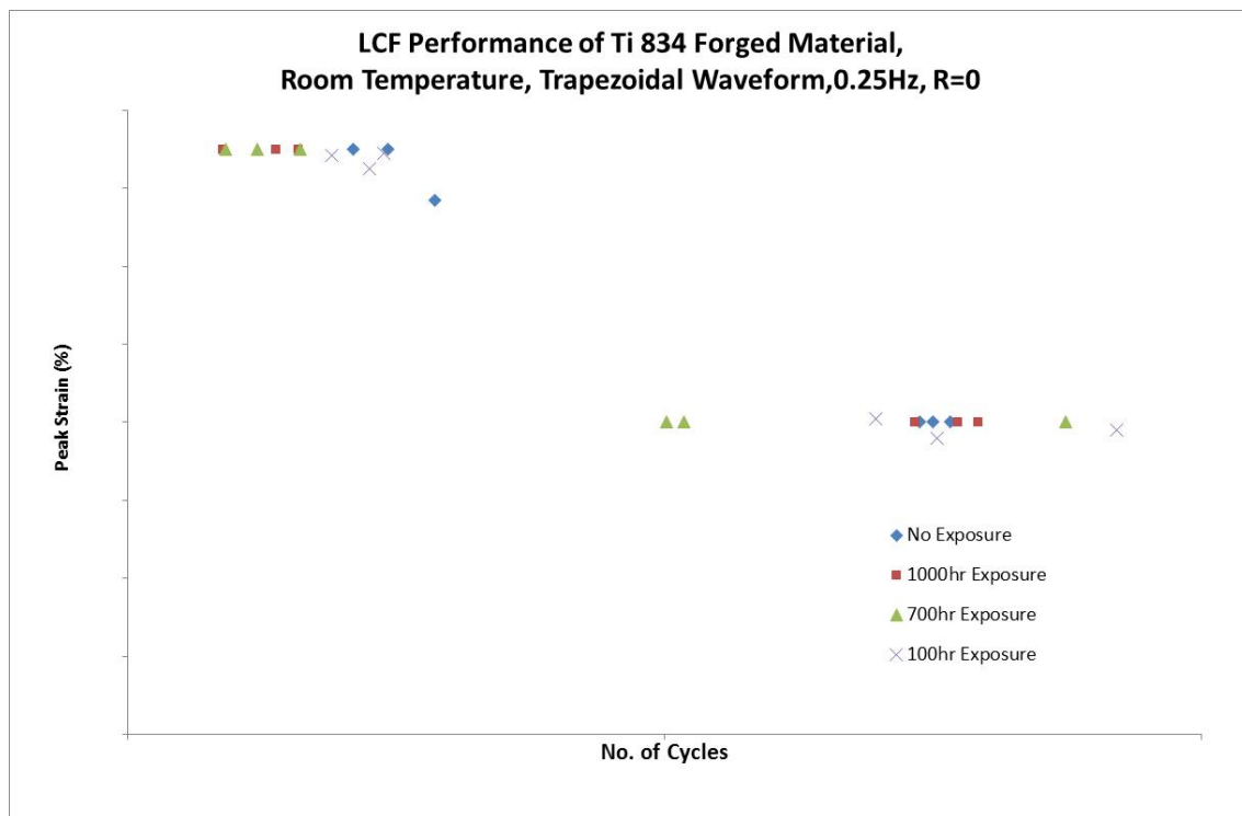
Figure 34 Room temperature peak strain versus cycles to failure for Ti-834 forged material
