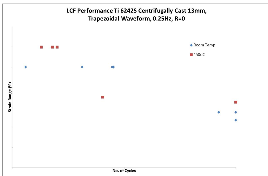
Figure 29 Peak strain versus cycles to failure for Ti-6242S 13mm product
