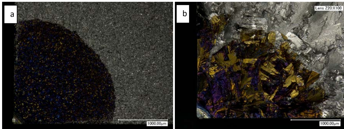
Figure 43 Crack path of a) Ti-834 forged material, b) Ti-834 centrifugally cast material
