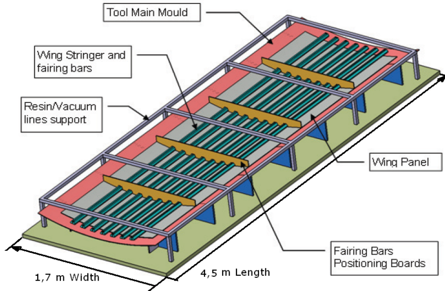
Figure 4 Test Bench concept design
