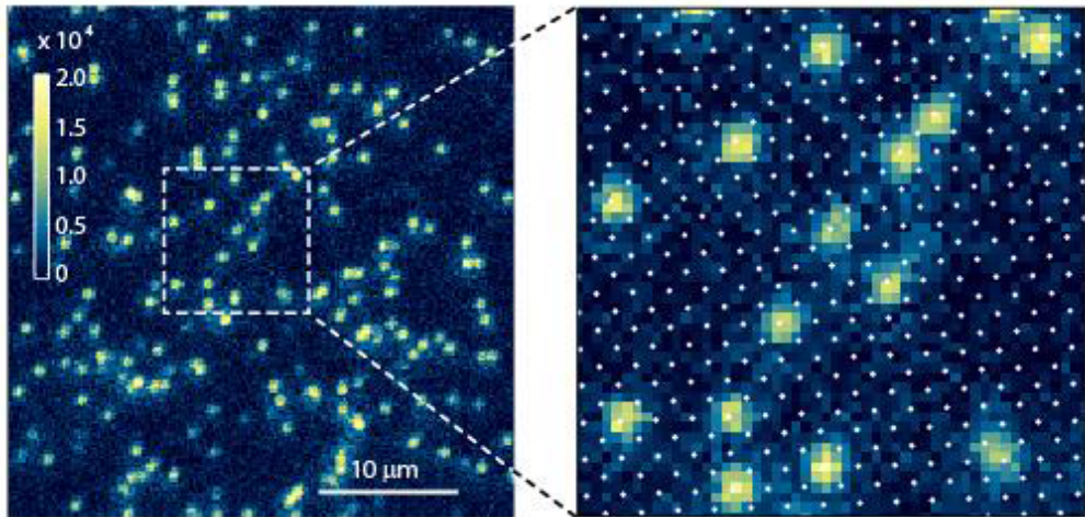
Figure 1, Fluorescence image of a dilute cloud of K 40 atoms in the optical lattice (left). White dots mark the lattice sites in a selected region (right) [E. Haller et al., arXiv:1503.02005]
