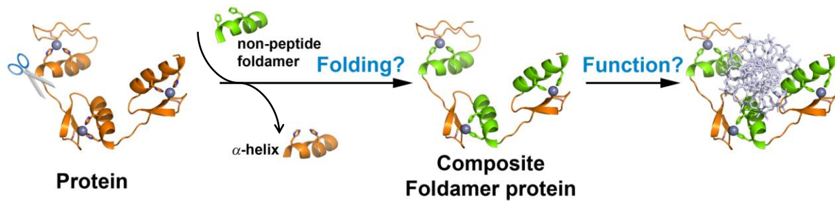
Fig. 1. Chimeric foldamer proteins generated by swapping one or several natural \alpha -helical domain with synthetic helical foldamers. Illustration of the concept with a 90 residue long protein with three zinc fingers : Zif268.
