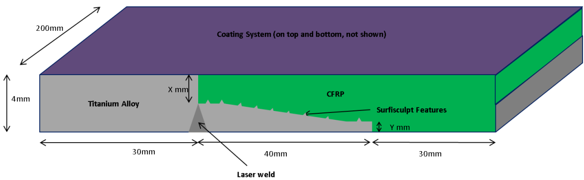
Figure 12: Component demonstrator (diagram not to scale)
