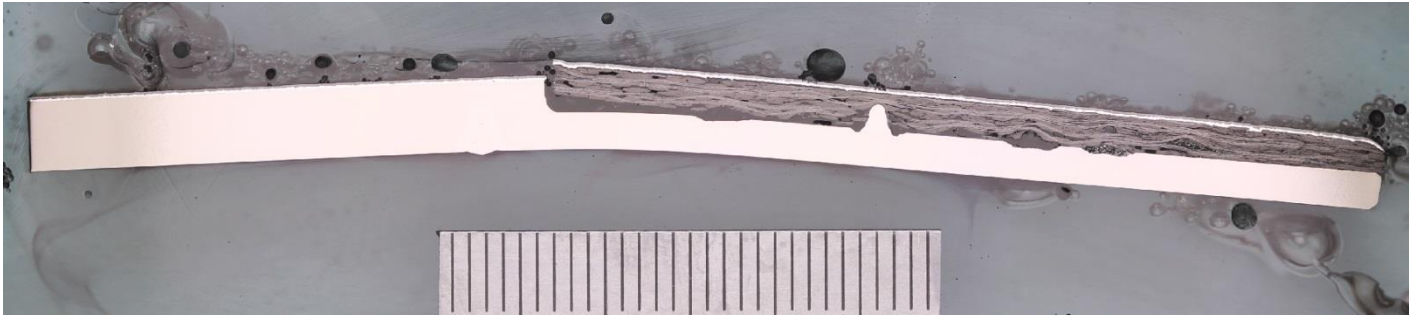
Figure 11: Cross-sections of 4-point bend testing samples after extraction. Photomacrograph of specimen TWI/20870/4 D11-1 (6mm displacement) after extraction and cross-sectioning showing detachment
