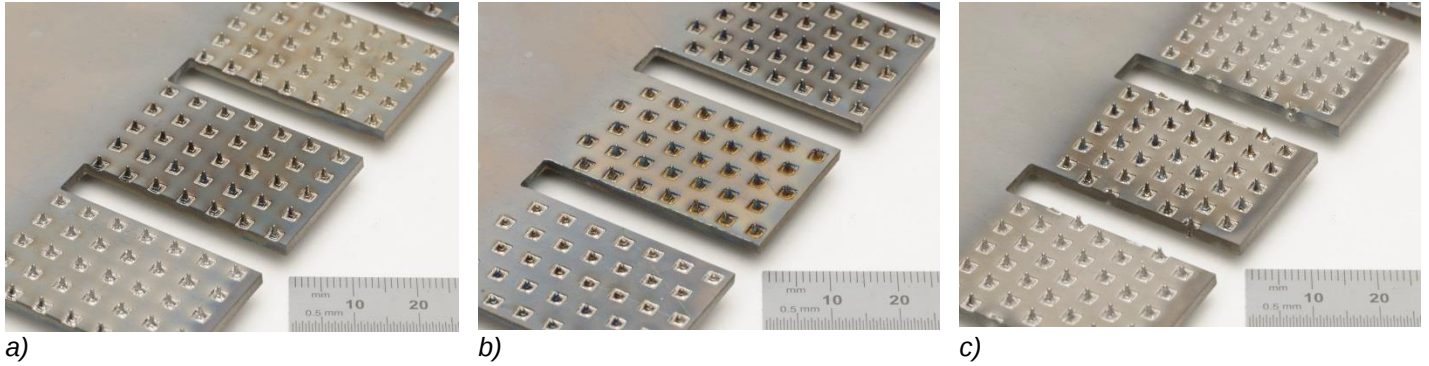
Figure 3 Image of the three different Surfi-Sculpt arrays on panel samples
