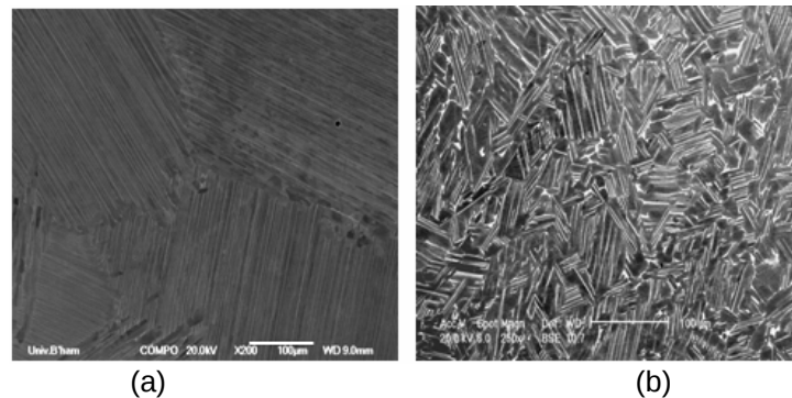
Figure 2: Back scattered scanning electron micrographs of samples of Ti46Al8Ta (a) as-cast and (b) cast and air cooled from 1360°C and subsequently HIPped at 1260°C for 2h illustrating the microstructural refinement that is achieved via this heat treatment [Courtesy: IRC-Birmingham].
