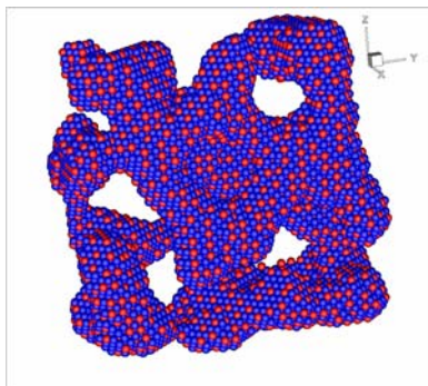
Figure 5: Computer simulation of the Ni-Al leaching process to produce nanoporous sponge Ni (Al-red Ni-blue).
