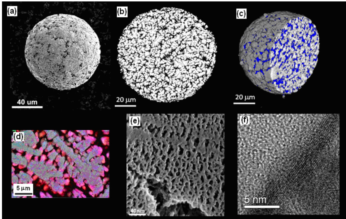
Figure 4: Structural hierarchy across 6 orders of magnitude: (a) a single gas-atomised sponge Ni powder particle after caustic leaching, (b) a cross-sectional micrograph showing the internal dendritic microstructure, (c) a 3D X-ray microtomograph from ESRF showing the internal porosity and connectivity in blue, (d) a compositional map of a leached dendrite, (e) the nanoporous sponge comprising \approx 5\text{-}10\text{nm} Ni crystallites, and (f) the nano-steps at the outer surface of the catalyst. [Courtesy: University of Ulm, Zeiss, CERAM Ltd. and ESRF/ESA].
