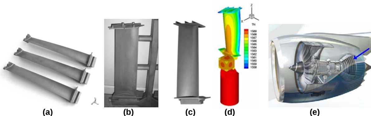
Figure 1: \gamma -TiAl-based low-pressure turbine blades centrifugally-cast at (a) ACCESS and (b) SETTAS-Doncasters, and tilt-cast at (c) IRC-Birmingham. (d) shows an example of heat and flow modelling applied to blade production (Greenwich University). (e) shows the end-user aero-engine turbine application (Rolls-Royce).
