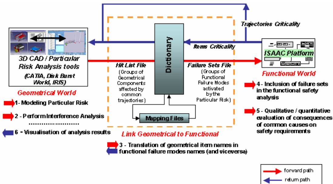
Figure 6 PRA Method
