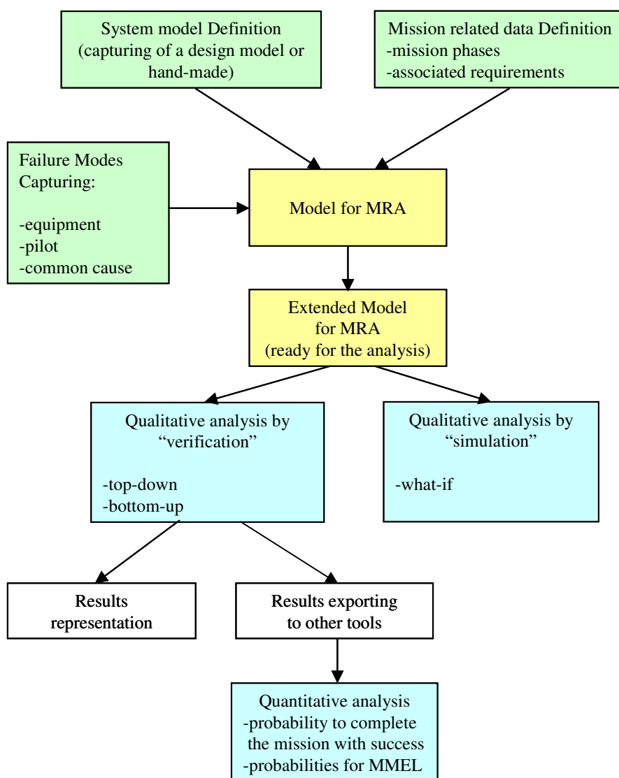
Figure 8 MRA methodology
