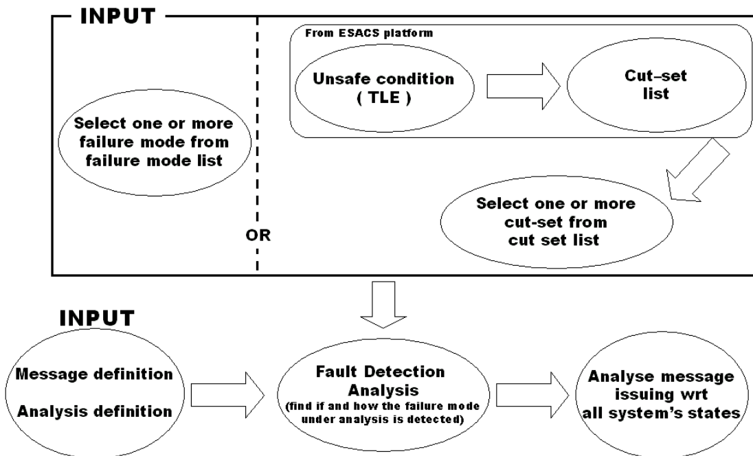
Figure 10 – Input/Output of fault detection analysis
