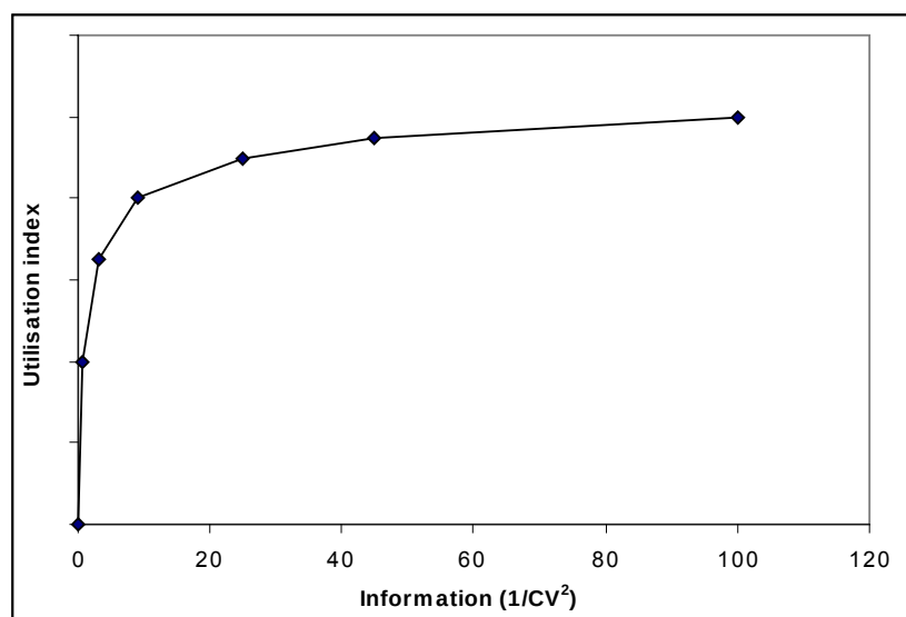
Figure 1. Relationship between an utilisation index (mean total catch) and information level ( 1/[CV]^2 of abundance estimates) for an MP, where each point along the curve represents roughly the same “risk of depletion”. [Adapted from Cooke 1999.]
