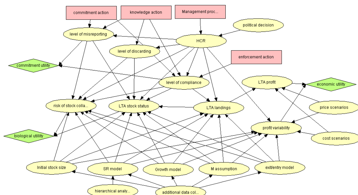
Figure 30 Example of the general BBN structure used to evaluate the value-of-information and the value-of-control and direct further analyses.
