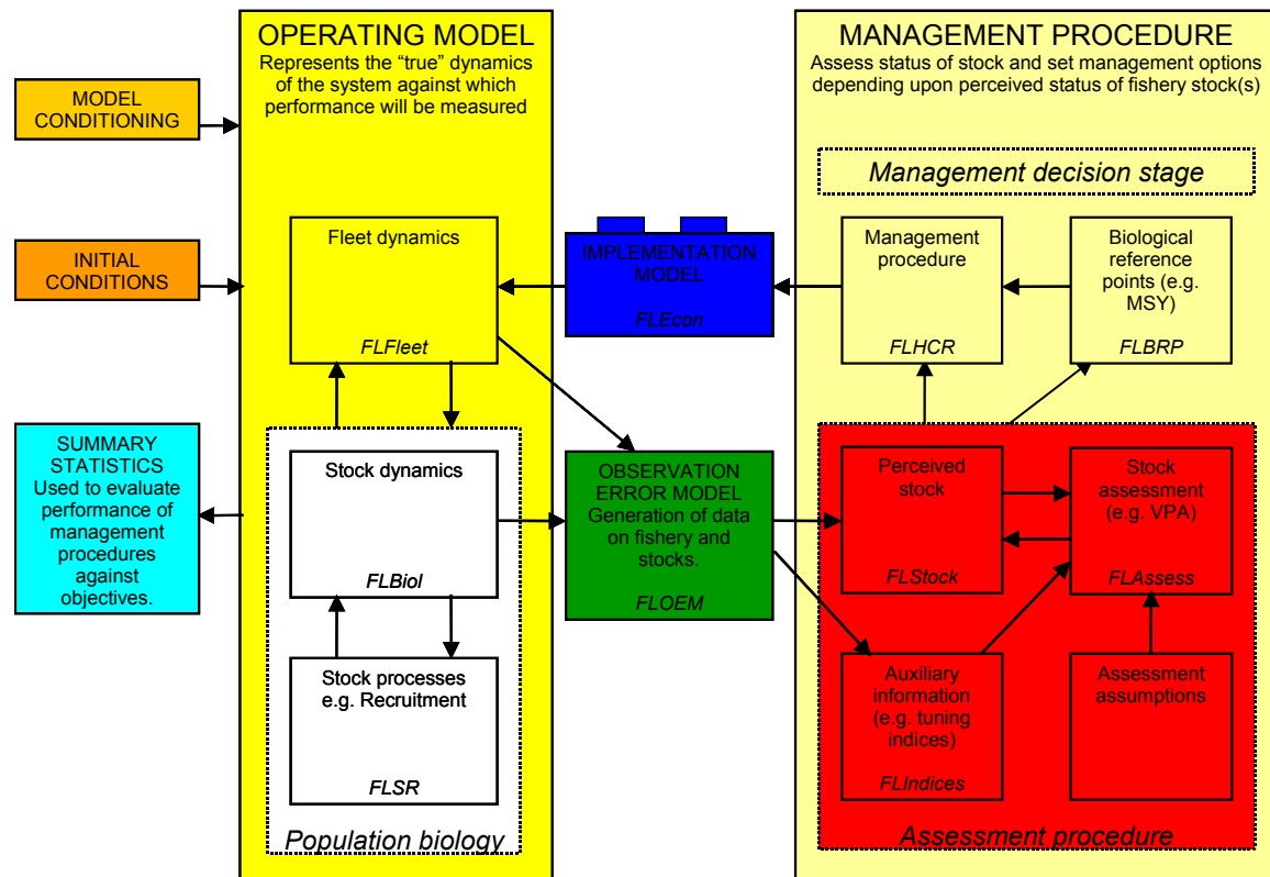
Figure 4. The FLR components that represent the elements required for the full-feed-back Management Strategy Evaluation framework.
