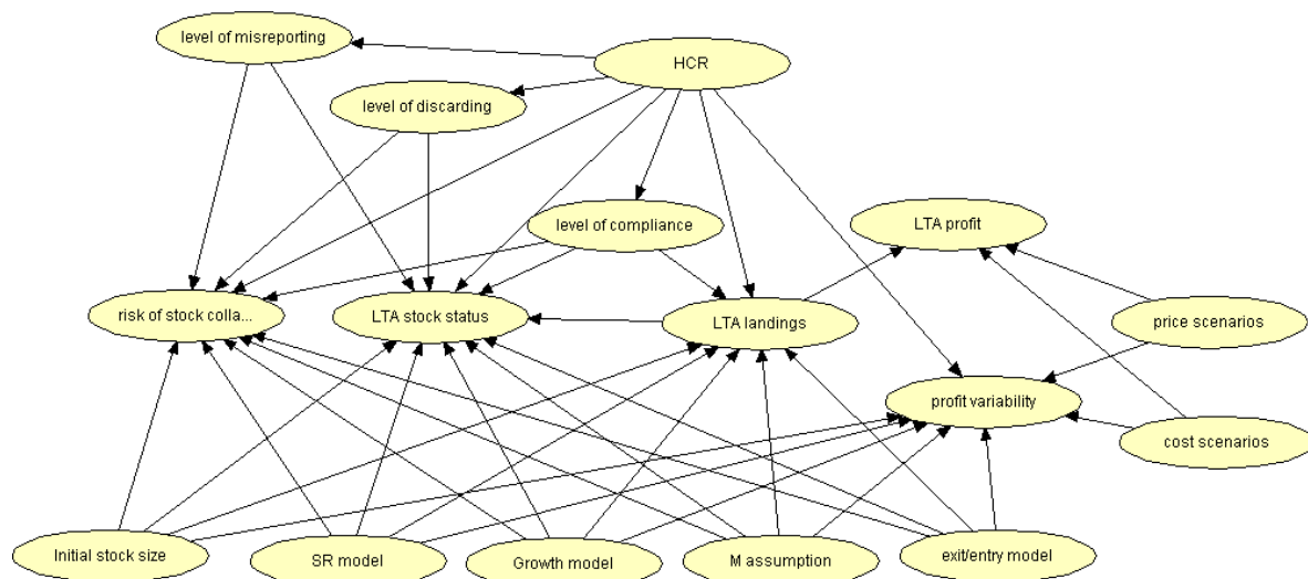
Figure 28: General structure for the BBN across case studies.
