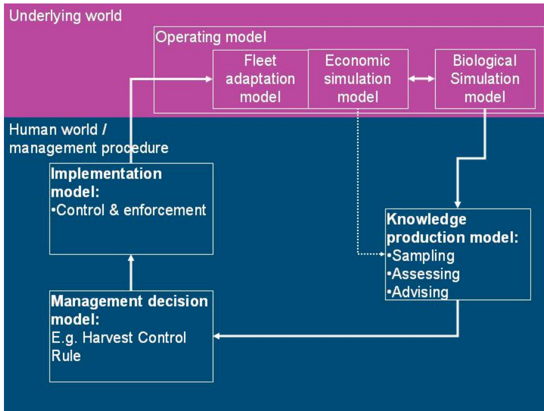
Figure 3. A conceptual diagram of the structure of the evaluation framework.
