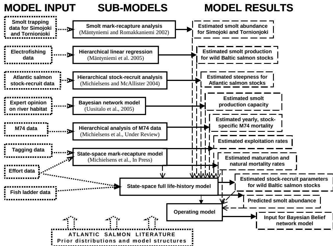
Figure 23 Conditioning of the operating model.
