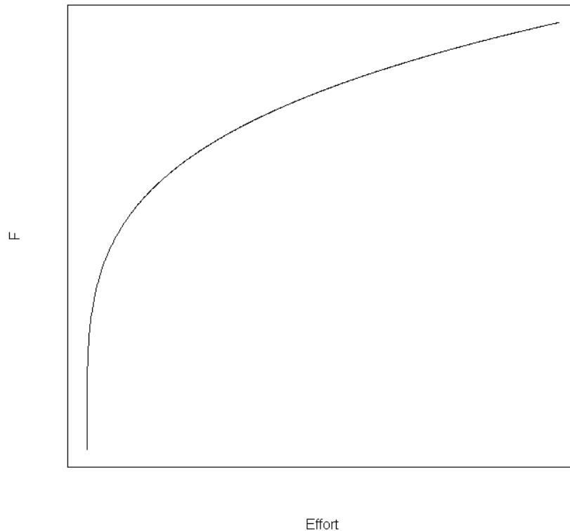
Figure 13. The expected relationship between effort and fishing mortality estimated in the case when days-at-sea becomes restrictive and fishermen reduce their number of less efficient trips.
