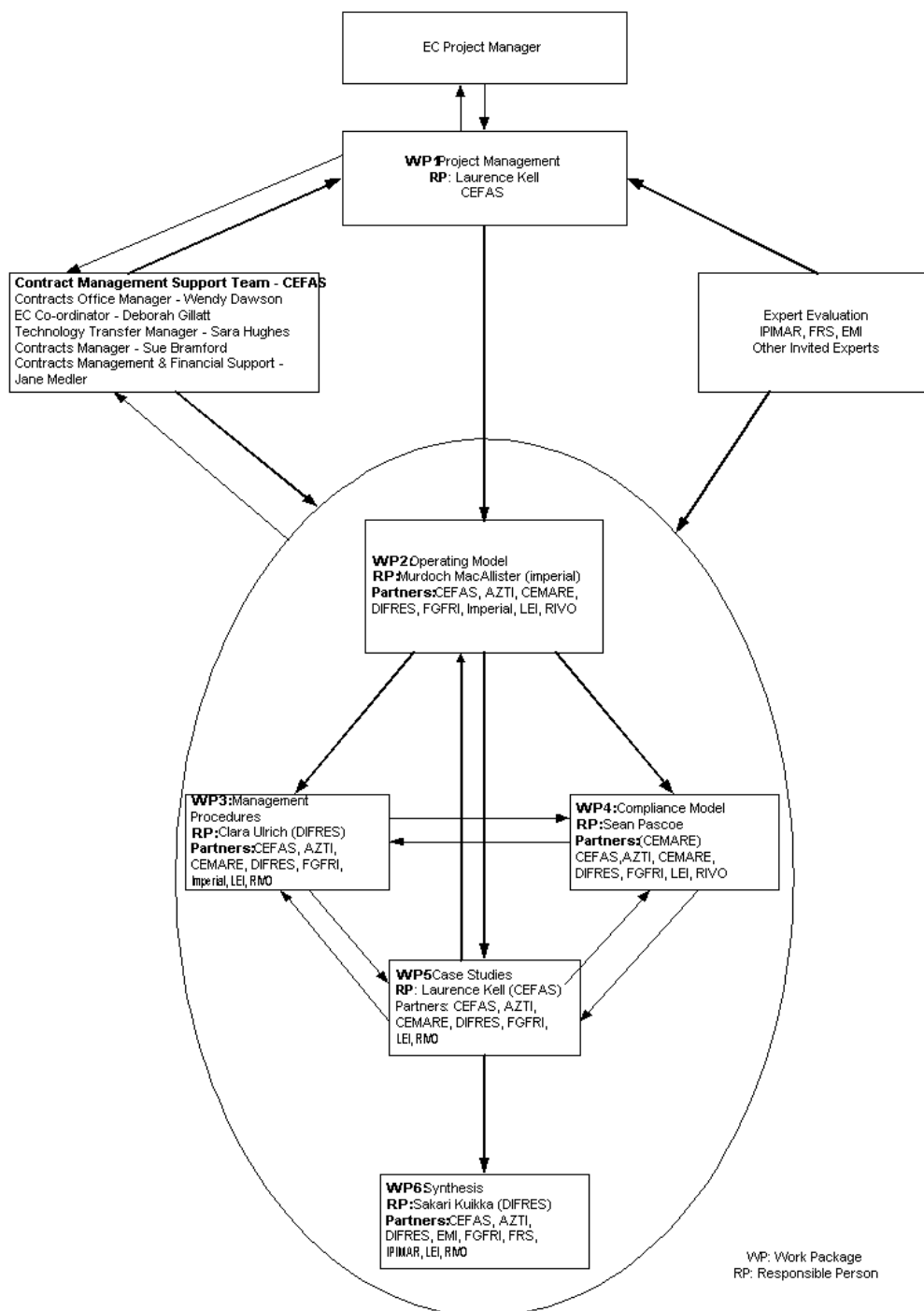
Figure 2. Project management structure including role of contractors
