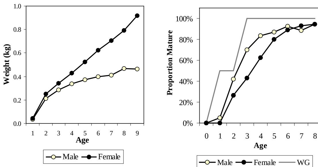
Figure 14. Mean weight- and proportion mature-at-age of male and female North Sea plaice.
