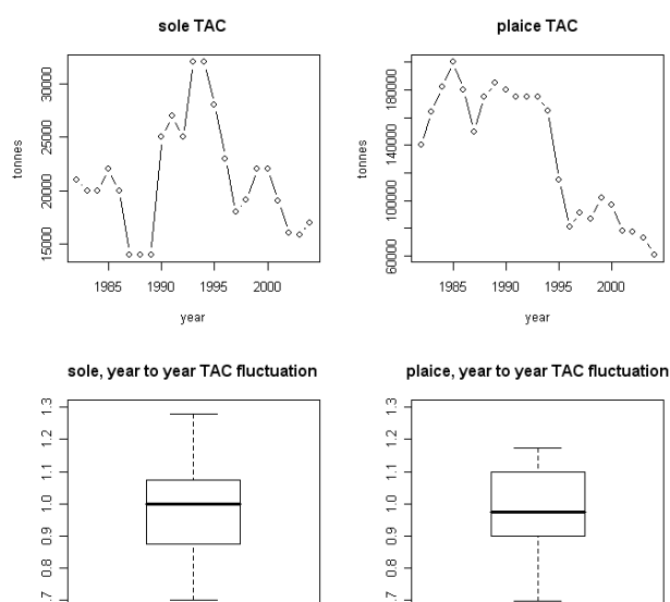
Figure 17. The TAC for both sole and plaice and the year to year variation in the TAC.
