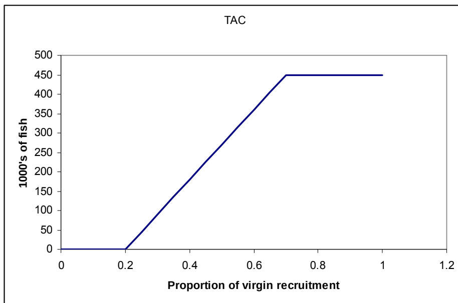
Figure 27. An example of a harvest control rule
