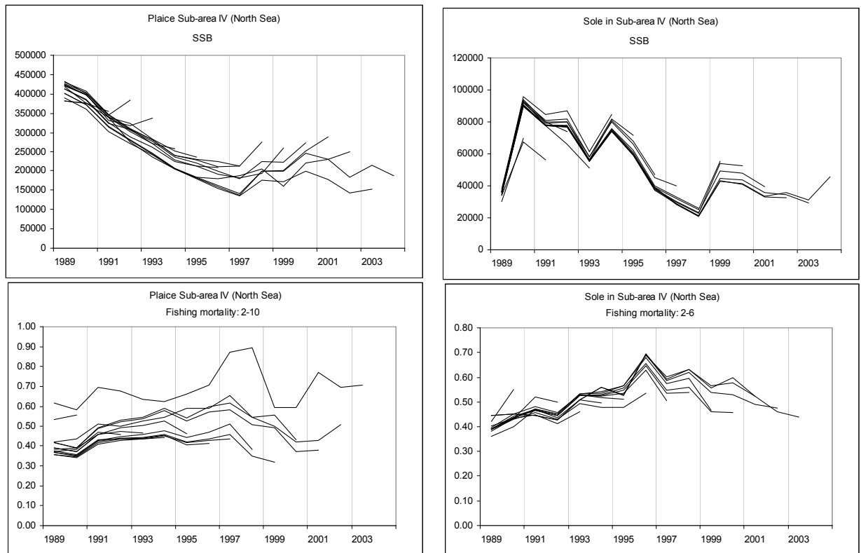
Figure 16. The trends of SSB and F for Plaice and Sole in the North Sea
