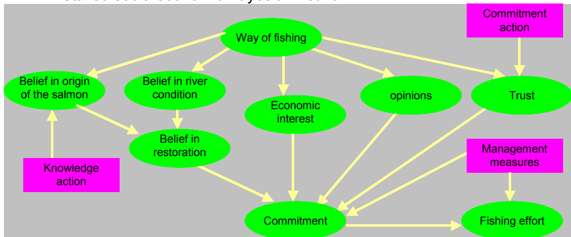
Figure 26. A simplified Bayesian Belief Network diagram describing the main factors behind the commitment of the salmon fishermen (P. Haapasaari et al. , 2005).
