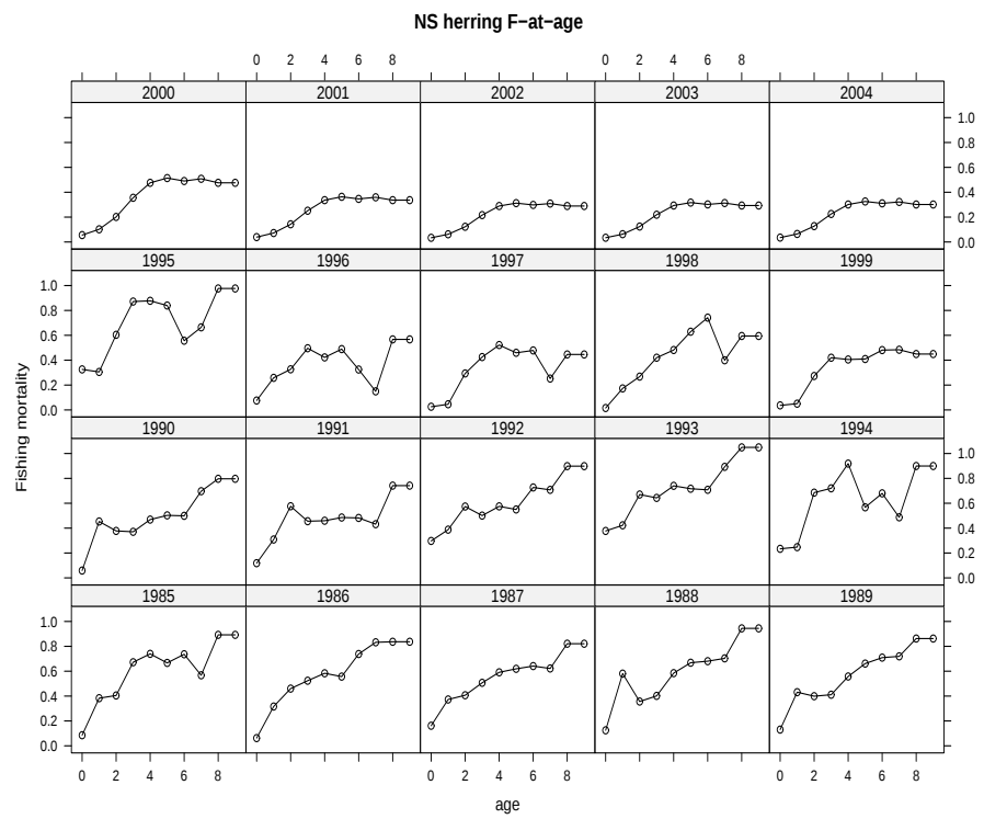
Figure 1: Lattice plot of the estimated fishing mortality-at-age for the North Sea herring stock.
