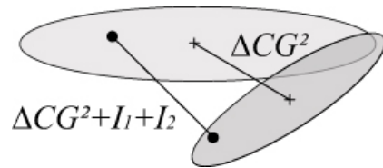
Figure 4.5.1. Collocation of two spatial populations, represented by two ellipses showing their center of gravity and their inertia, is measured with the GIC through specific distances.
