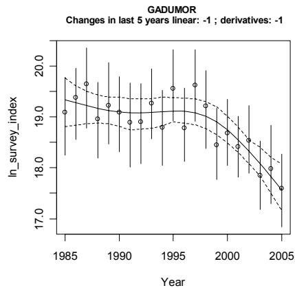
Figure 5.7.4. Ln-transformed survey time series with fitted smoothed model (GAM). Header provides direction of changes as found by fitting a linear slope over the 5 most recent years, and by the proposed method, referred to as ‘derivatives’. This information is repeated in the table.
