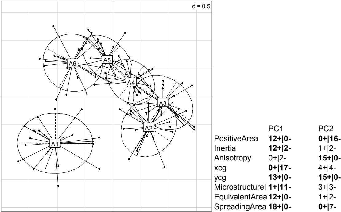
Figure 5.11.1. Left: MFA representation of each age in each year (points) relatively to the age gravity centre. Right: Spatial indicators that are the most correlated to the first two principal axes
