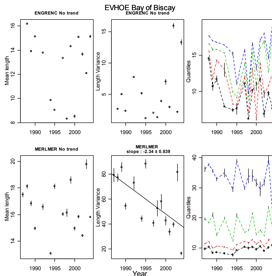
Figure 3.6.1: Time series of indicators for Bay of Biscay anchovy (code= ENGREN) and hake (code= MERLMER) with long term trends. Data from the IFREMER EVHOE demersal trawl survey of the Bay of Biscay.
