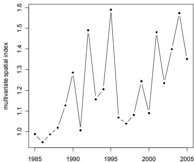
Figure 5.11.2. Monitoring North Sea cod in the sub-space of the two first principal MFA axes using the spatial indicators (Fisboat Table 1) : time series of the multivariate distance representing the deviation of the stock from its reference spatial distribution all ages considered.
