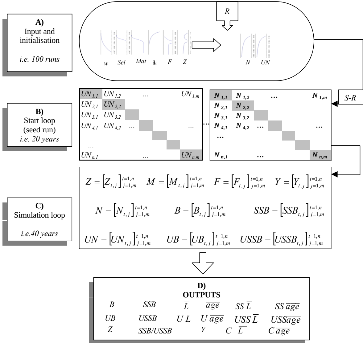
Fig. 1 – Scheme of the Aladym-r tool. R =recruitment; w =individual weight; Sel =selectivity; Mat =maturity; M =natural mortality; F =fishing mortality, Z =total mortality; N =exploited population, UN =unexploited population, B =exploited biomass, SSB =exploited spawning stock biomass, UB =unexploited biomass, USSB =unexploited spawning stock biomass, S-R =stock-recruitment relationship, Y =yield, t =time, j =cohort.
