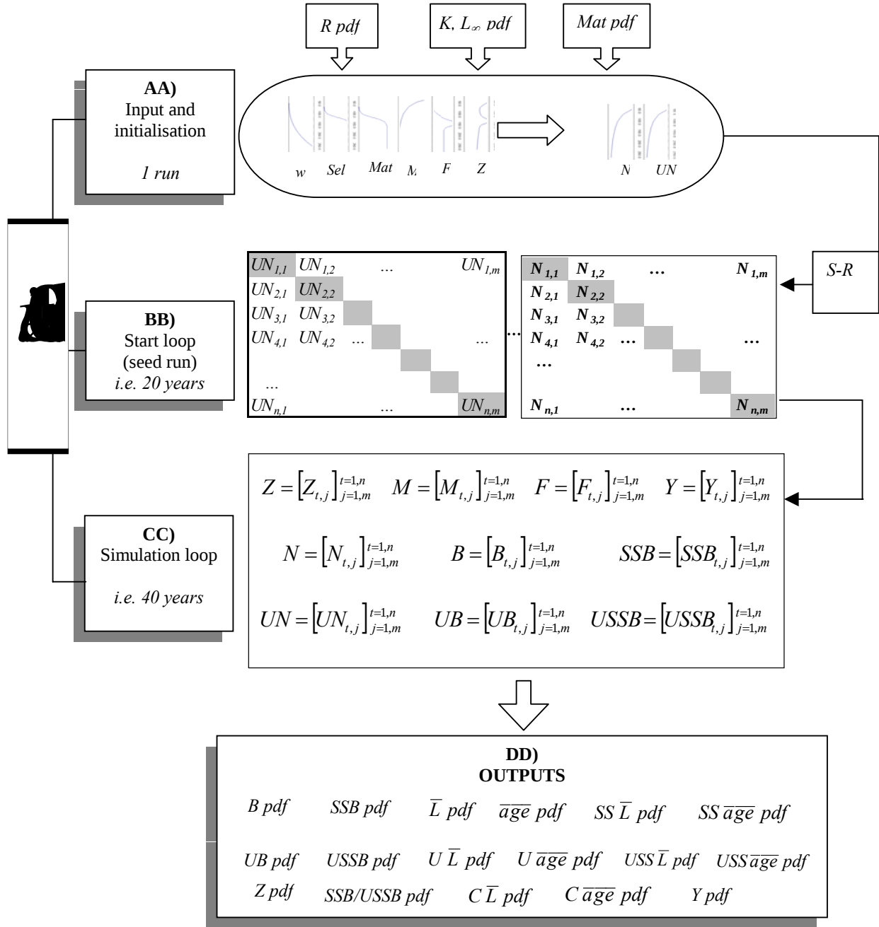
Fig. 2 – Scheme of the Aladym-q tool. pdf =probability distribution function; K , L_{\infty} growth parameters, R =recruitment; w =individual weight; Sel =selectivity; Mat =maturity; M =natural mortality; F =fishing mortality, Z =total mortality; N =exploited population, UN =unexploited population, B =exploited biomass, SSB =exploited spawning stock biomass, UB =unexploited biomass, USSB =unexploited spawning stock biomass, S-R =stock-recruitment relationship; \bar{L} = average length ; \overline{age} = average age ; SS =exploited spawner's population; USS =unexploited spawner's population; C =capture in numbers; Y =yield, t =time, j =cohort.
