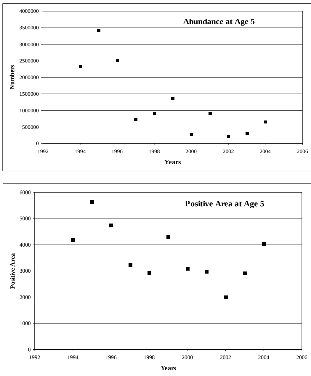
Fig.4a: Time series of the indices that convey the major signal in the evolution of Baltic Sea cod. Indices are Abundance at age 5 and Positive area at age 5.
