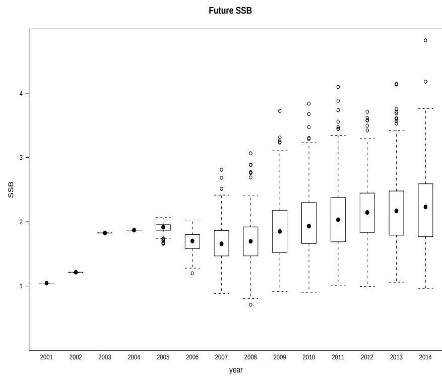
Figure 2: Boxplot of the past and future SSB for the North Sea herring stock under a particular management scenario.
