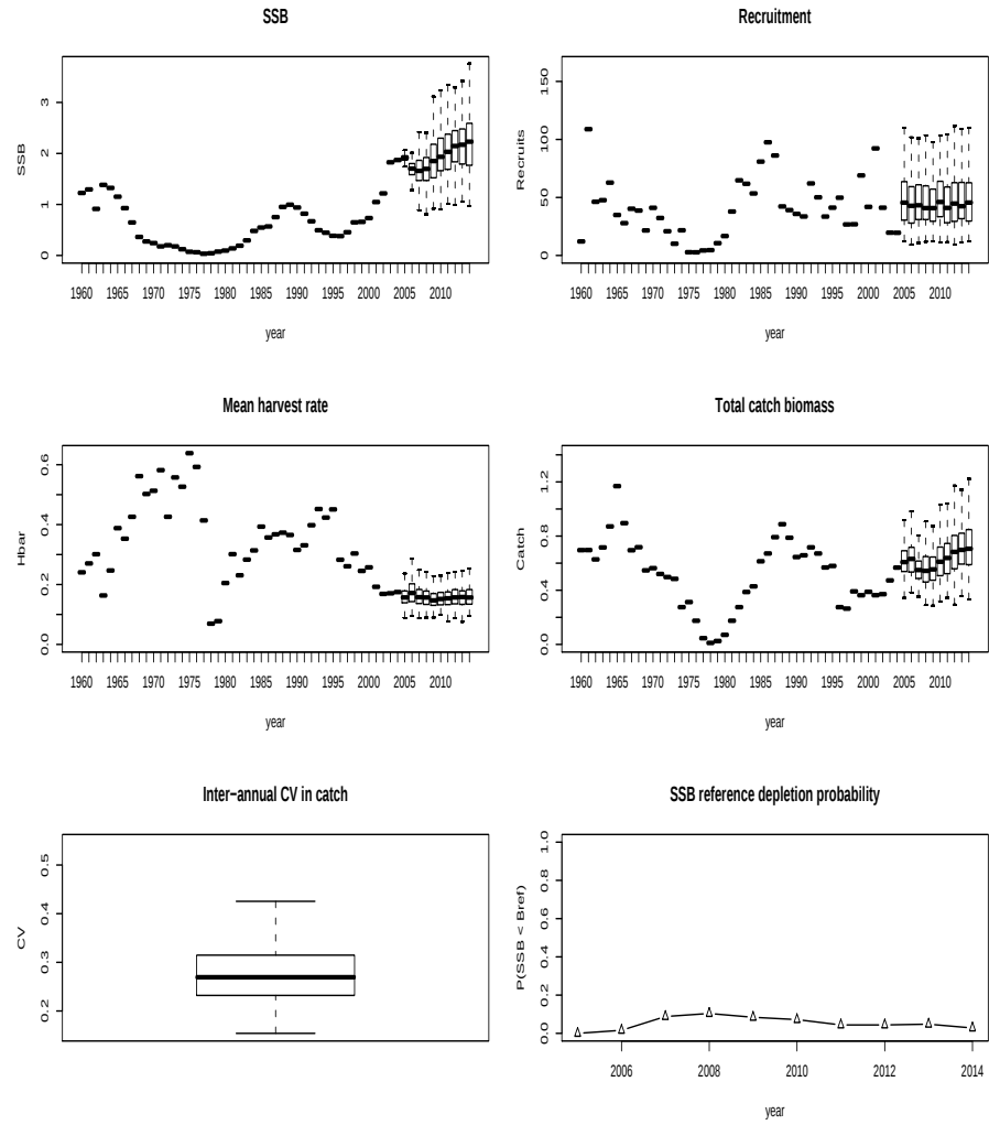
Figure 3: The FISBOAT management scenario summary plot which is documented and a feature of the FLFisboat package.
