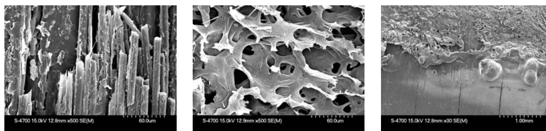
Fig. 23:. Typical damage morphology of CF/PPS at the surface impacted by the laser (Nd:YAG)_CIDAUT
