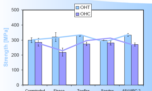
Fig4: mechanical results on TP NCF (LTSM+ Airbus-F)
