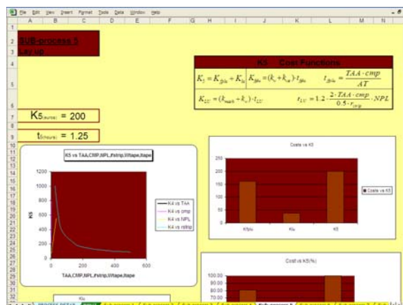
Fig 38: High Speed Lay-Up process cost analysis, sub-process 5 cost estimation (LTSM)
