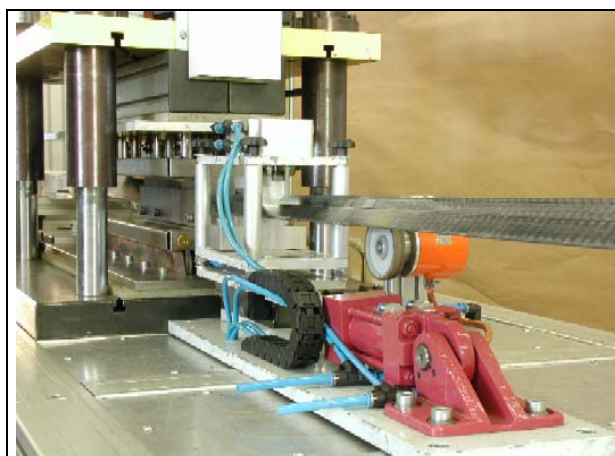
Fig 18: ACM continuous forming machine
