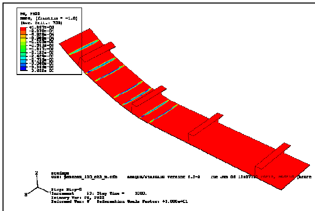
Figure 1.2.4.4 Local mechanical simulation Displacement x 10
