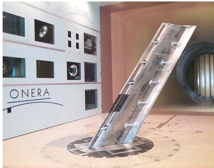
Figure 5. AFV 3-element configuration for transition studies in the ONERA F1
