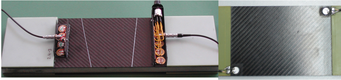
Fig. 7 left: Reusable transducer arrays, generating straight wave fronts right: Glued PZT patches (PCL 255 \varnothing 10 \times 0,5 ) at optimized positions
