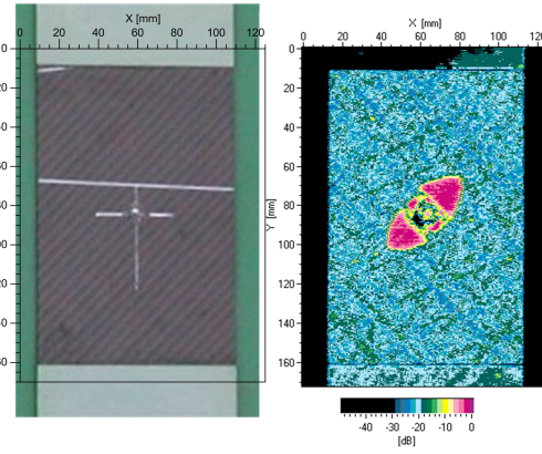
Fig. 9: Photo and ultrasonic C-scan after 20 Joules impact
