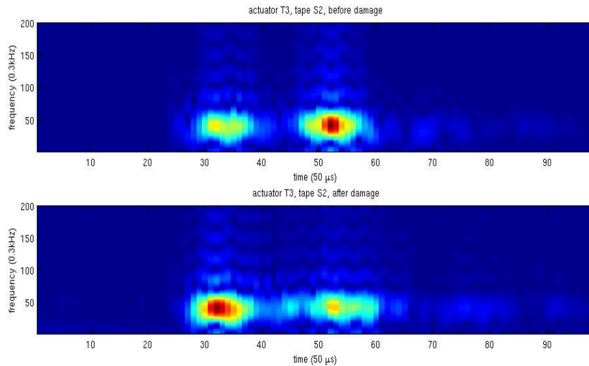
Fig. 24 The time frequency images of the signals obtained using the optical fibre S2, and the actuator T3, before and after the impact was made. The frequency of the signal is 12 kHz, length of the signal arrays is N=25000 , window size W=500 , l=250 .
