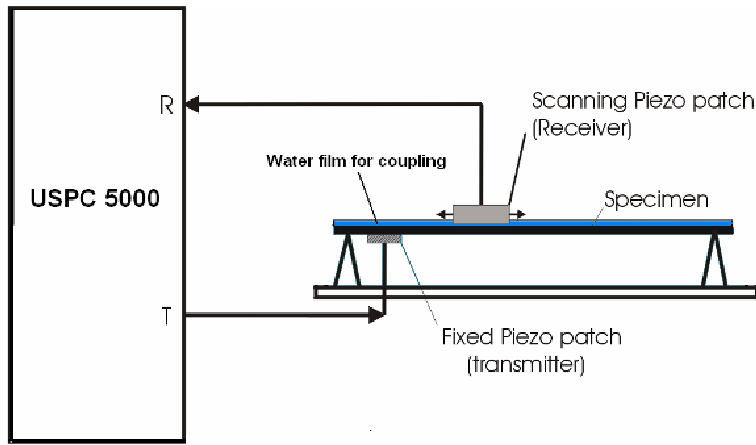
Fig. 4: Experimental setup for wave visualisation with direct coupling
