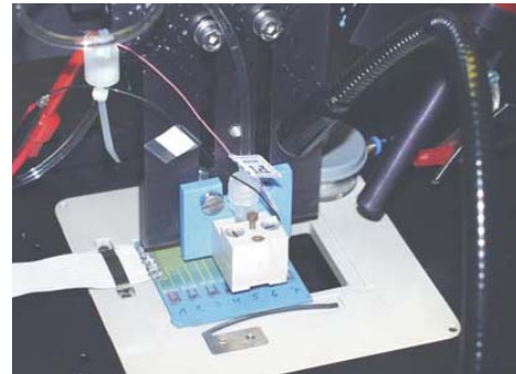
Fig.2: At the heart of the GaNano instrument is an arrangement of seven labelled sensors on a translation stage that are able to analyse droplets with a volume of 50 \mu l to 1 nl.
