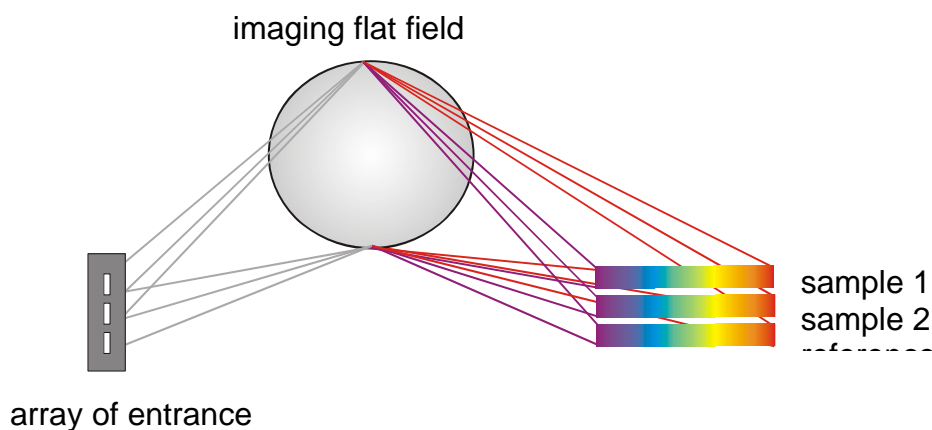
Fig.8: Scheme of a multi-channel spectrophotometer
