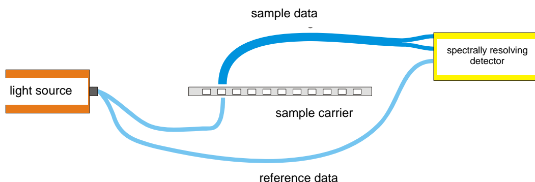
Fig.7: Scheme of the nanoliter spectrophotometer
