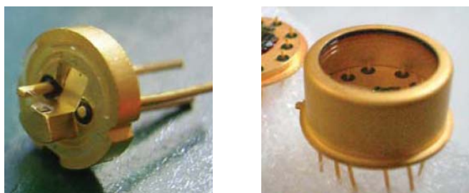
Fig.4: The GaNano system features GaN-based lasers (left) and detectors (right).
