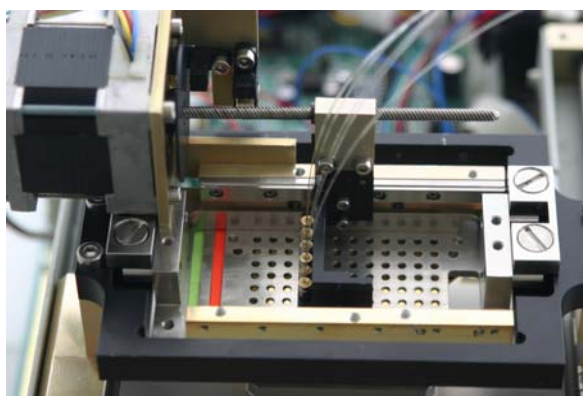
Fig.6: Fiberoptic Scanner used in the real-time PCR device of AJ, based on the “SpeedCycler” – the high speed thermocycler of AJ
