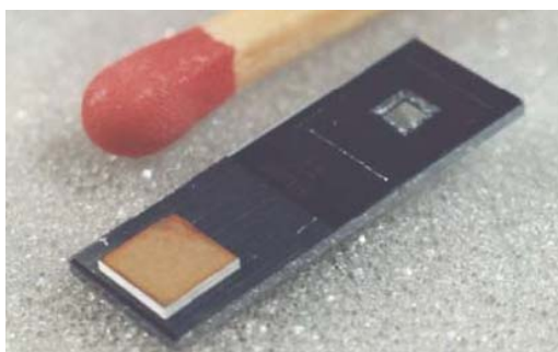
Fig.3: Droplets are applied to the sensors with a silicon device that uses microchannels and pumps driven by piezoelectric actuators.
