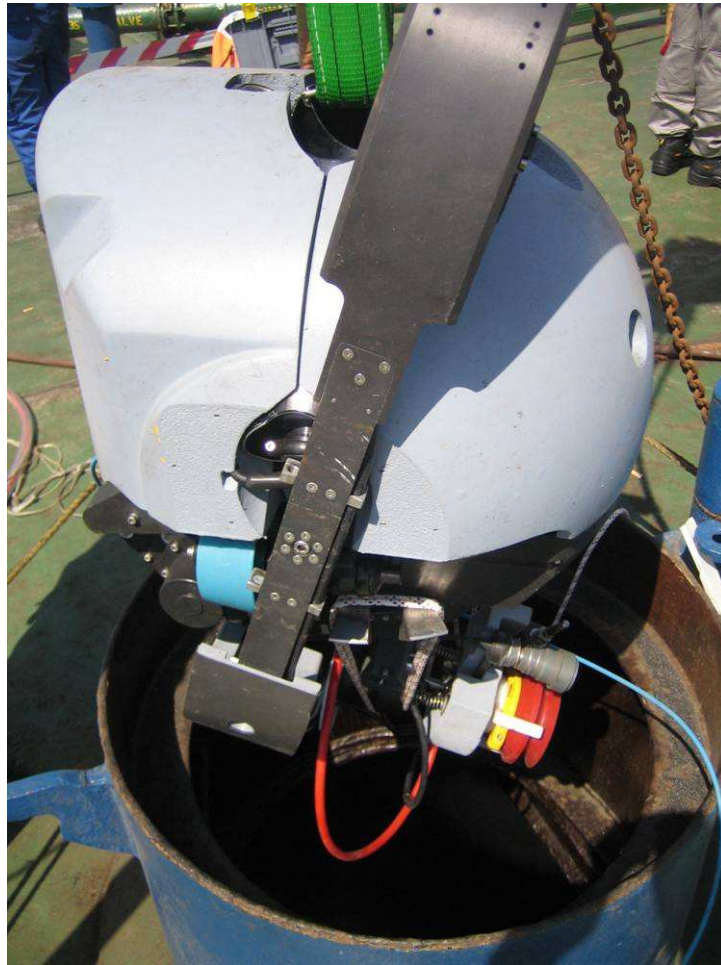
Figure 4 Inserting the ROV into the flooded ballast tank
