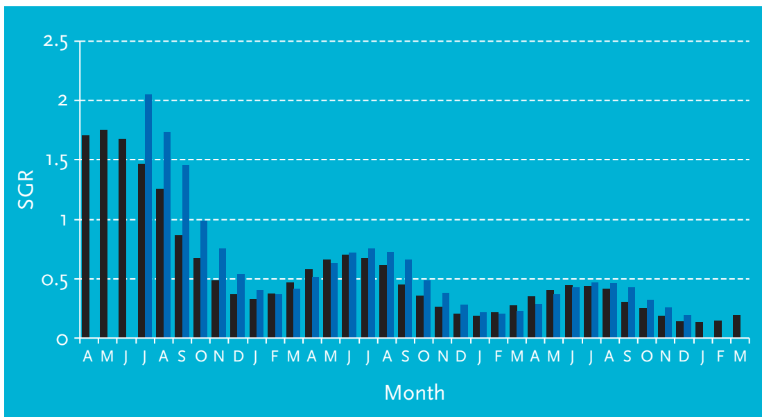
◆ FIGURE 55. Specific Growth Rate (SGR) prediction using Thermal Growth Coefficient (TGC) model for Japanese Seabass (black) and Yellow croaker (blue), calculated on the basis of production and environmental data from Huangdun Bay.
