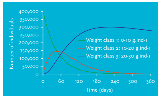
◆ FIGURE 91. Bivalve population model
