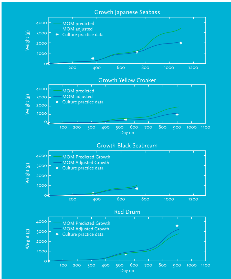
◆ FIGURE 57. Daily values of growth of Japanese Seabass, Yellow Croaker, Black Seabream and Red Drum simulated with MOM fish sub-model and compared to data of harvest weights.
