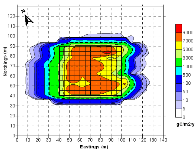
Figure 5. Screening model for carbon input to sediments from fish culture.
