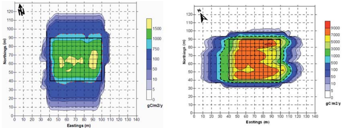
◆ FIGURE 95. Modelled particulate carbon input to sediments ( \text{g C m}^{-2} \text{y}^{-1} ) from fish culture at the Demonstration Site in Huangdun Bay under ambient current flow conditions (left), and an illustration of how dispersion for the same production level may change under slower hydrodynamic conditions (right).
