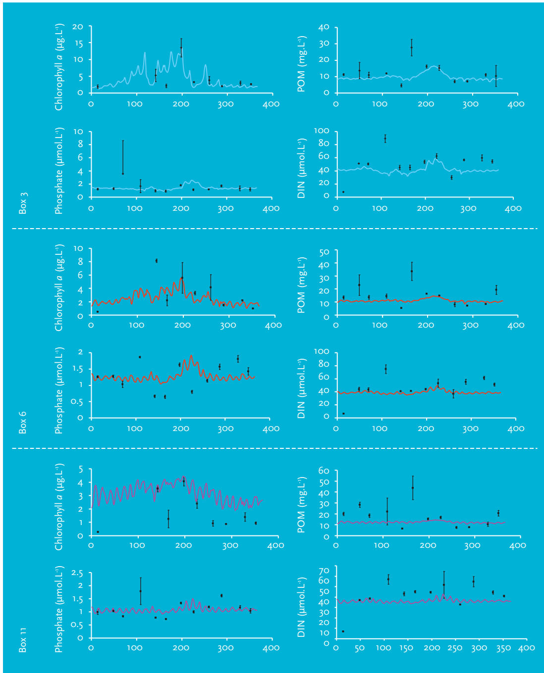
◆ FIGURE 8o. Results for Xiangshan Gang EcoWin2000 boxes 3 (inner box Huangdun Bay), 6 (middle box), 11 (outer box), plotted with average daily data (2005/6).
