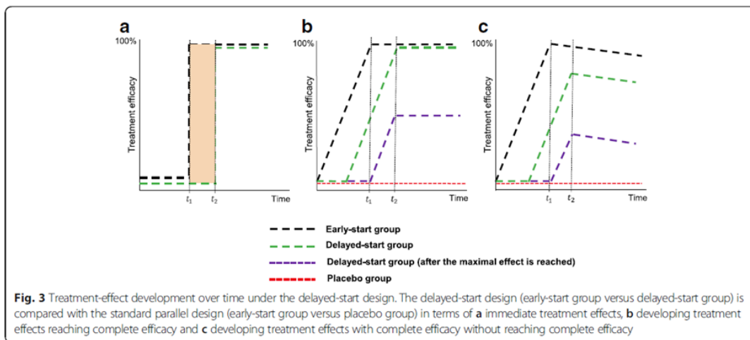
Figure 6. Graphical illustration consequences of delayed-start design.
