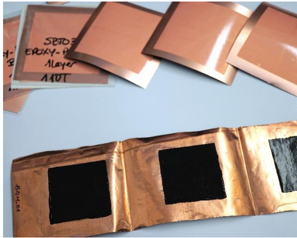
Screen printed high-k dielectric composite (top) and screen printed high conductivity elastomer electrode (bottom)
