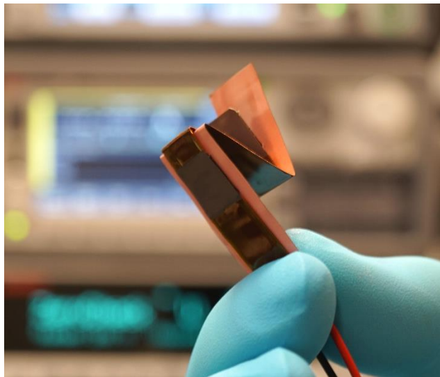
Harvester device folded foils for stacking
