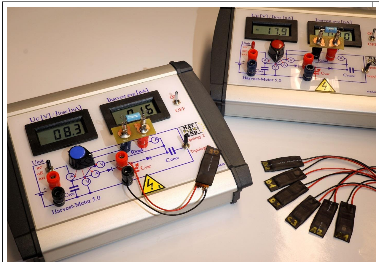
Harvester characterization device
