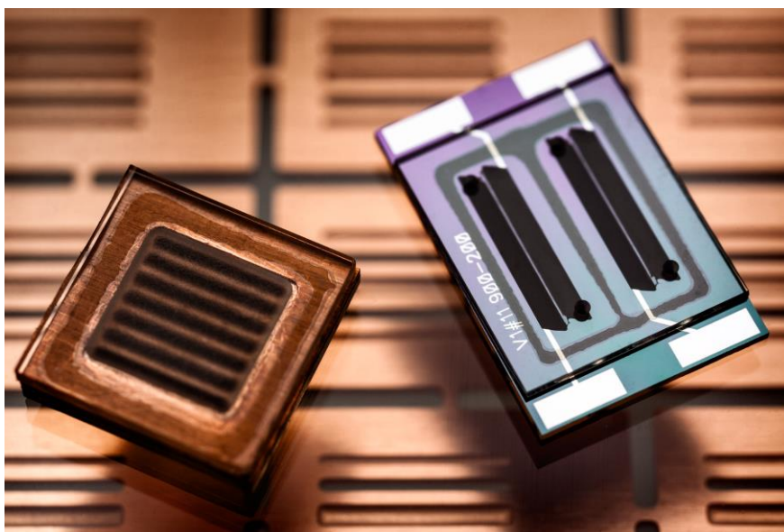
MATFLEXEND lithium ion battery with interdigitated electrodes
