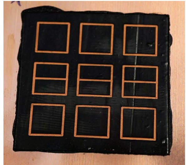
Screen printed high conductivity elastomer with device patterning
