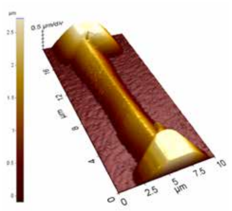
Novel SThM-AFM method for determining thermal properties of a single Si-NW
