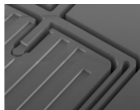
SEM picture of Si springs, patterned electret and shock absorbers
