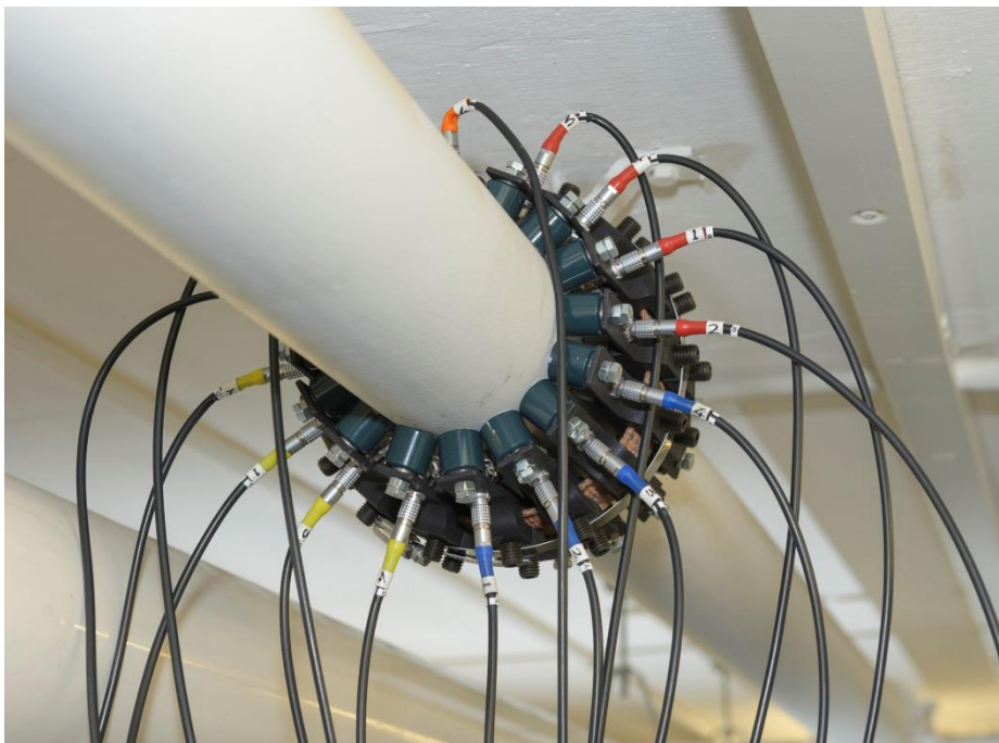
Figure 4. SprinkTest transducer array deployment system (collar).
