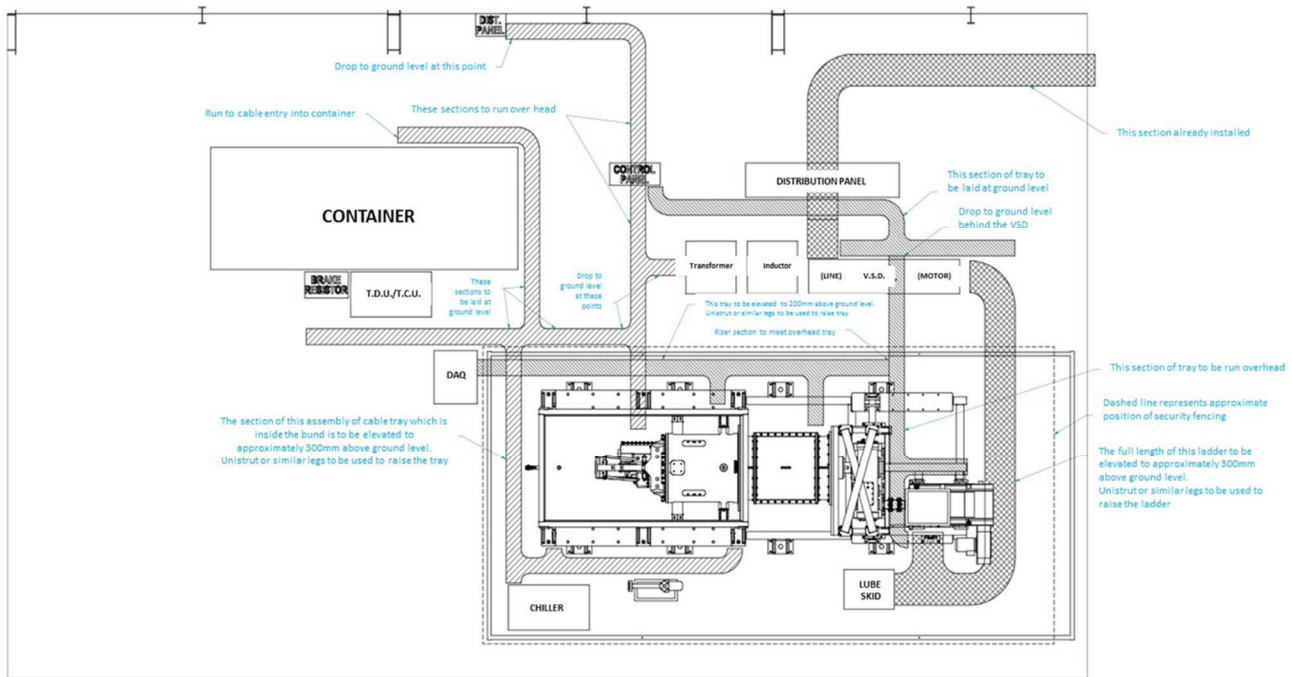
Figure 30: Containment Layout
