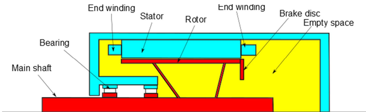
Figure 7: Cross section of turbine T2
