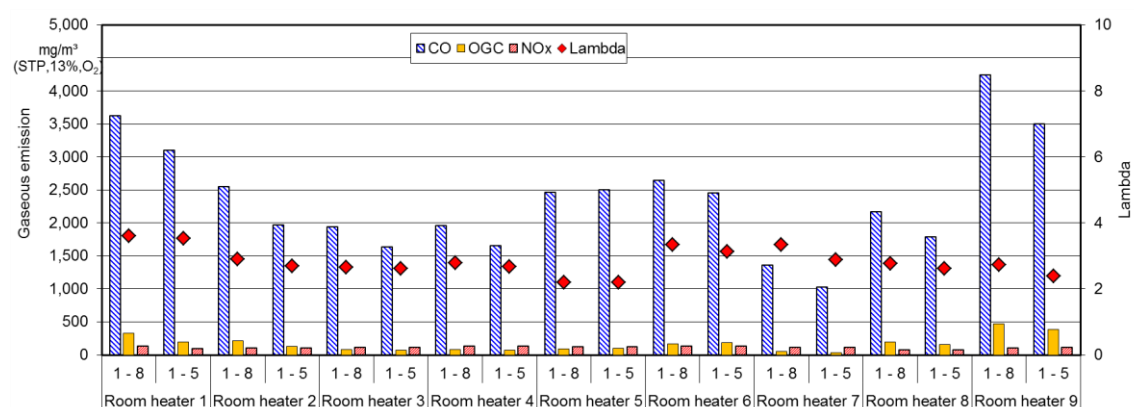
Figure 14: Mean values of validation measurements for beReal tests, evaluated for nominal load batches (1-5) and nominal and part load batches (1-8), for CO, OGC, NOx and lambda at all 9 firewood room heaters (n = 3 repetitions)
