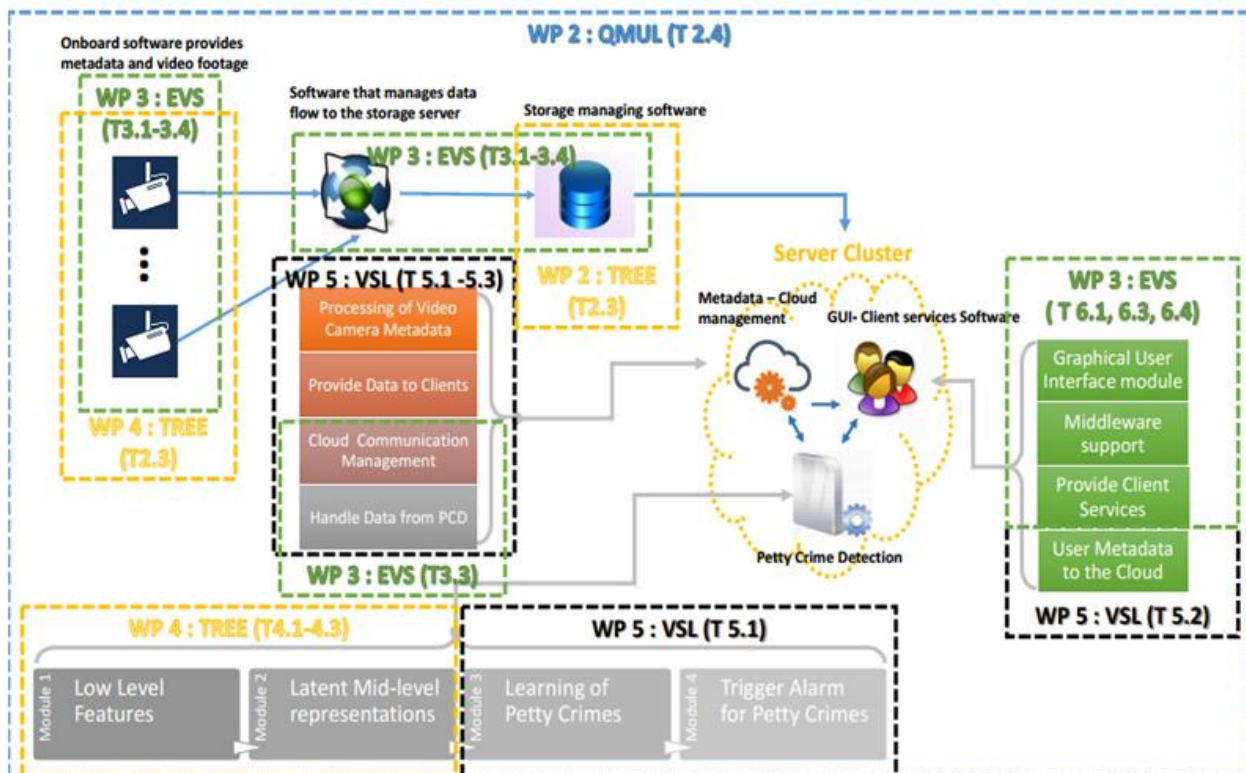
Figure 3. SmartPrevent Software Pipeline architecture.
