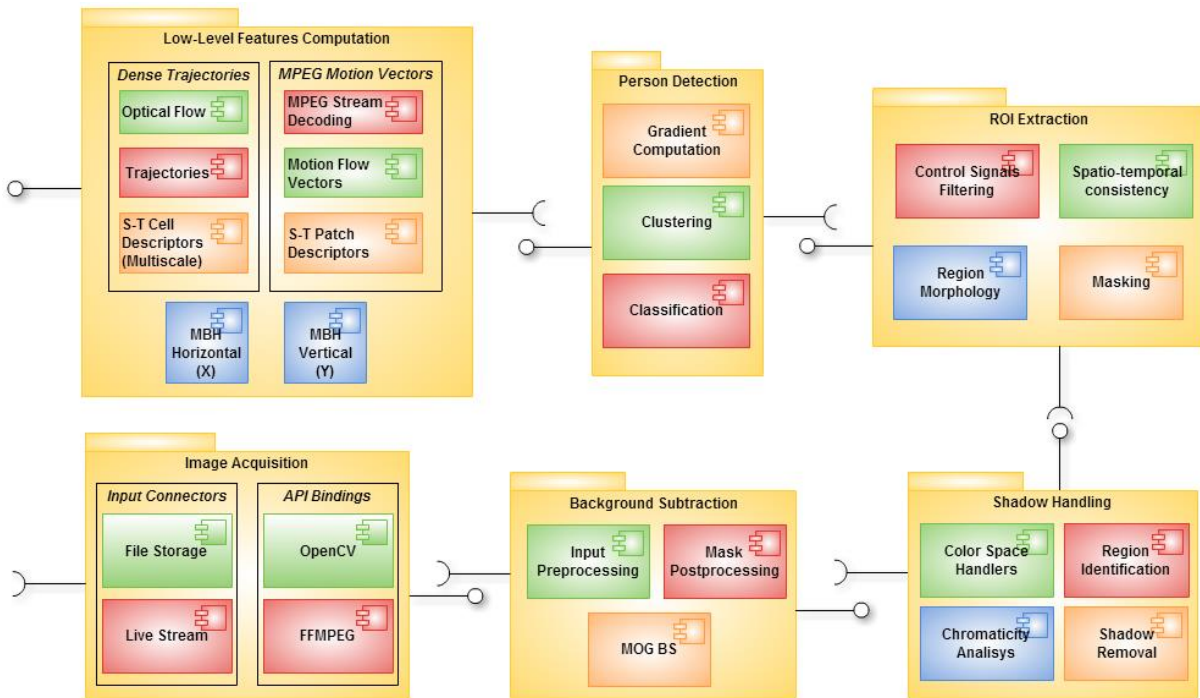
Figure 5. Overview of the final software packages of the low-level scene understanding pipeline. For each package, its top-level modules are also shown.
