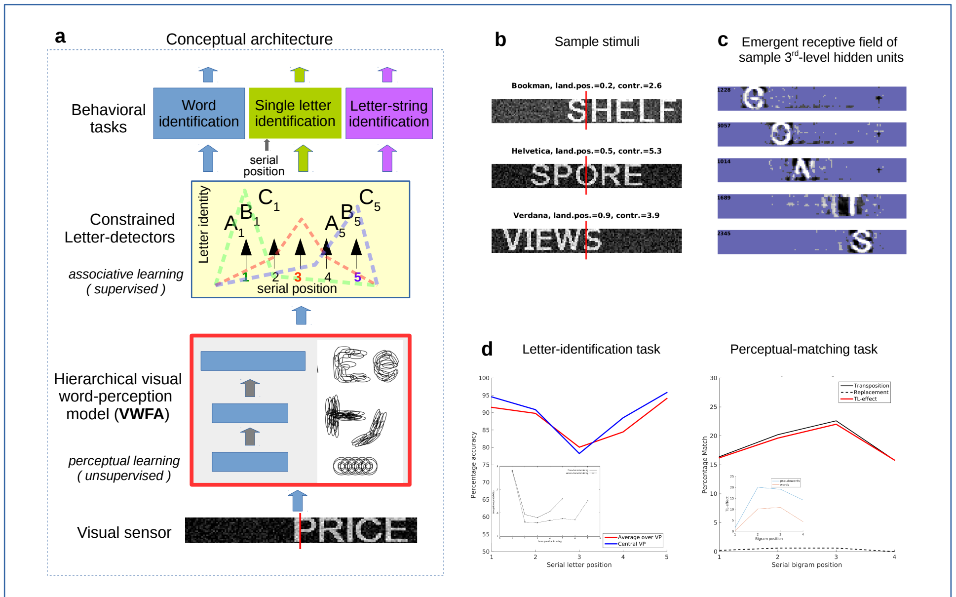
Figure 1. The Visual Front End of Reading (a) neurocomputational model of visual word perception. (b) Samples stimuli at different contrasts and viewing positions. (c) Sample emergent detectors of the letters at different serial positions. (d) Uncertainty of serial position measured through letter-identification and perceptual-matching explains behavioral effects such as neglecting letter transposition.
